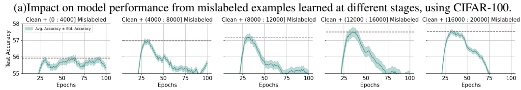
Figure 6: Impact of mislabeled samples learned at different stages on model generalization performance.
