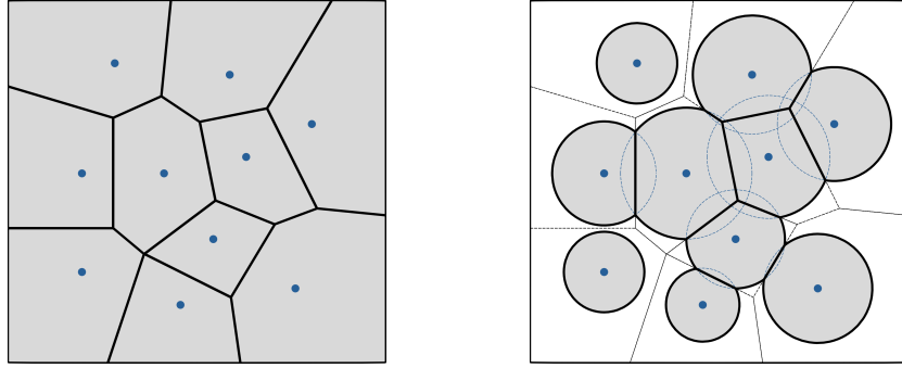
Figure 1: (left) Voronoi cells, and (right) restricted Voronoi cells
