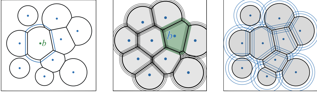
Figure 2: (left) The \delta -expanded restricted Voronoi cell of RV_y^\delta(b) , (middle) in a \delta -feasible transport plan, the point b \in B can transport mass to its 2\delta -expanded restricted Voronoi cell, (right) the decomposition \mathcal{X}_\delta .
