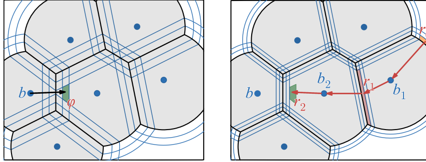
Figure 3: (left) In scale 2\delta , the point b transports mass to a region \varphi inside its 4\delta -expanded Voronoi cell, and (right) in scale \delta , the \varphi becomes a violating deficit region. A consolidating path \langle r_0, b_1, r_1, b_2, r_2 \rangle can be used to bring this deficit to the exterior of the restricted Voronoi cells.
