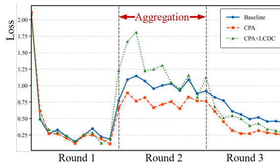
Figure 6: Visualization of loss curves.
