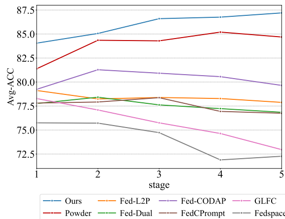
Figure 3: Avg-ACC curves on the seen tasks across training stages .
