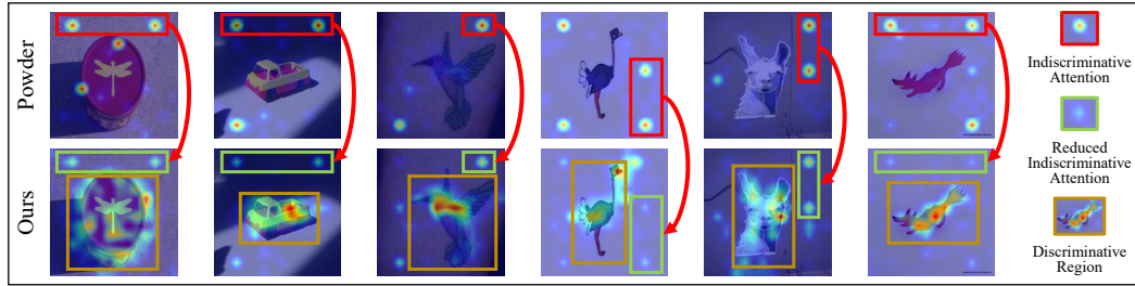
Figure 5: Visualization of attention across prompt and image regions.
