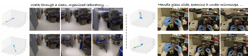
Figure 6: Visualizations demonstrate that EgoDreamer can generate various egocentric videos based on different low-level commands, where the left-side poses denotes the kinematic movements in 3D space (from blue to red).
