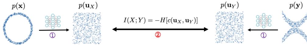
Figure 1: Overview of the proposed vector copula-based MI estimator (VCE) , which explicitly disentangles the modeling of marginal distribution and dependence structure (i.e., the vector copula). VCE first respectively computes the vector ranks \mathbf{u}_X and \mathbf{u}_Y corresponding to the two marginal variables X and Y with flow models (①). It then finds the vector copula c \in \mathcal{C} from the vector copula pool \mathcal{C} that best matches with the joint distribution p(\mathbf{u}_X, \mathbf{u}_Y) of the estimated vector ranks (②). Mutual information I(X; Y) is computed as the negative differential entropy of the vector copula c , which itself is irrelevant to the two marginal distributions p(\mathbf{x}) and p(\mathbf{y}) .
