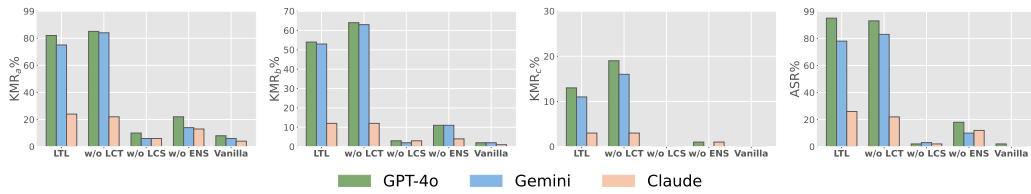
Figure 9: Ablation on our two proposed strategies: Local-level matching and ensemble, conducted by separately removing local crop of target image (LCT), local crop of source image (LCS), and ensemble (ENS). Removing LCT has only a marginal impact.
