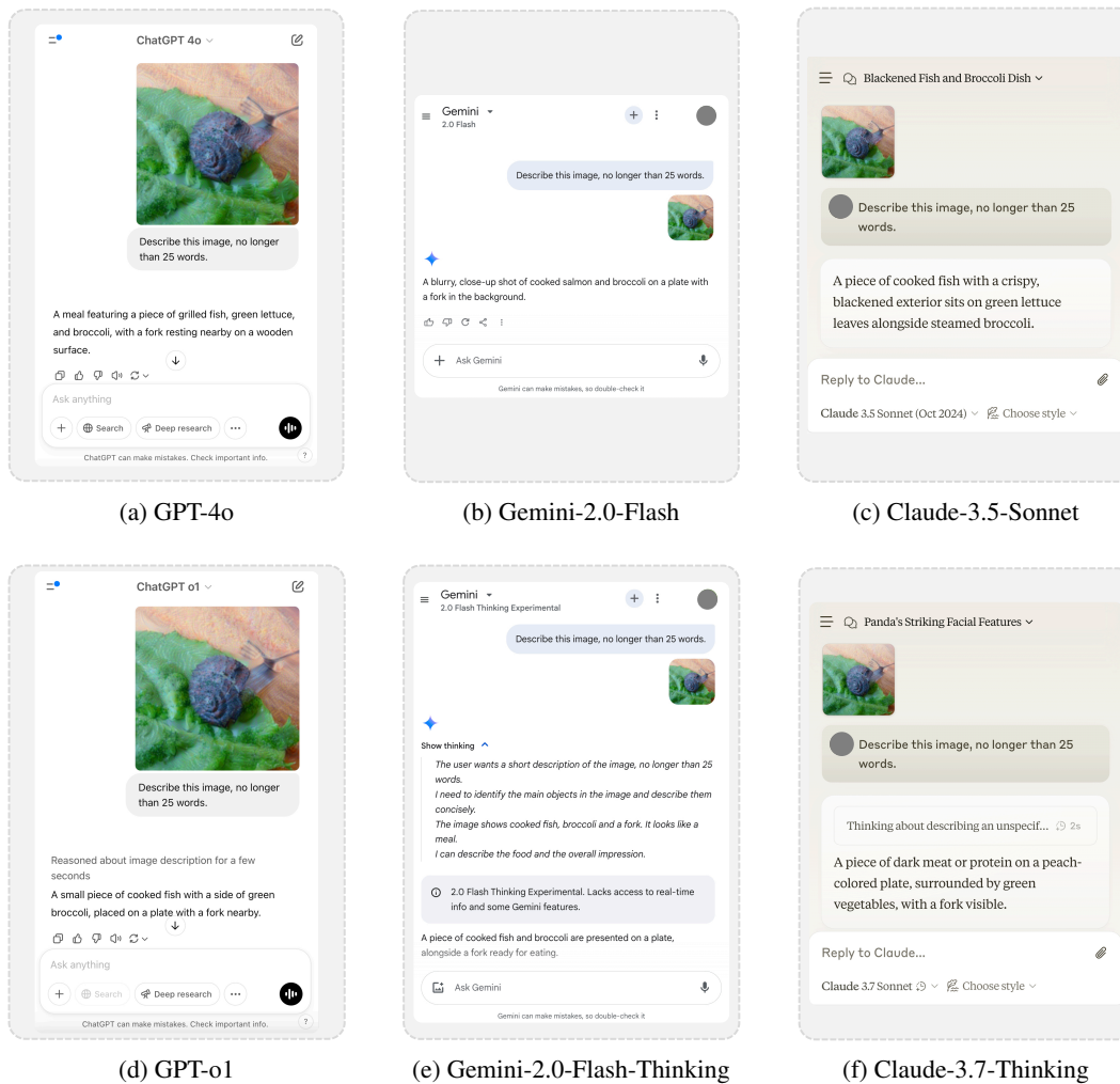
Figure 16: Example responses from closed-source commercial LLMs to targeted attacks generated by our method.
