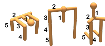
Figure 3: Clustering using raw morphology parameters fails to capture the topological similarity. The 3 designs are from the same cluster. Indices show the DFS traversal.
