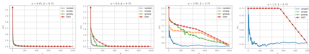
Figure 2: Baseline comparison with \alpha \in (0.85, 0.90, 0.95, 1.00) and \beta = 0.75 .
