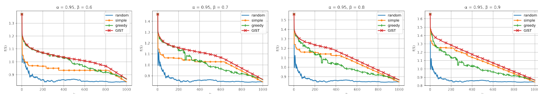
Figure 3: Baseline comparison with \alpha = 0.95 and \beta \in (0.60, 0.70, 0.80, 0.90) .
