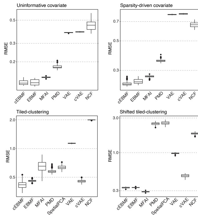
Figure 2: Performance of the different matrix factorization methods in the simulated data sets. Each boxplot summarizes the root mean squared errors (RMSEs) across 100 simulations in that scenario. (Lower RMSEs are better.) See Figures 5–8 in the Appendix for additional results from the simulations. Note Fig. 1 shows results from one of the tiled-clustering simulations in detail.
