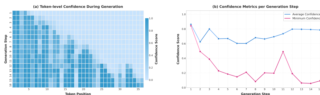
Figure 1: Overview of model confidence dynamics during iterative generation. (a) Token-level confidence heatmap across token positions and generation steps (darker shades indicate higher confidence). (b) Average and minimum confidence scores per generation step. This visualization highlights the dynamic and non-uniform nature of model confidence that A-CFG aims to leverage.
