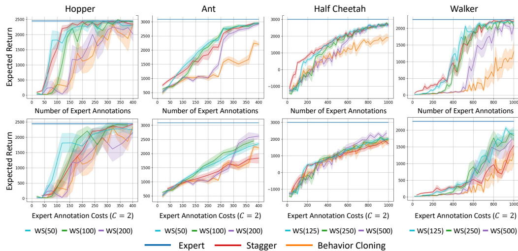
Figure 5: Performance comparison under MSE loss across MuJoCo tasks. Results show that WARM-STAGGER (WS) achieves comparable sample efficiency and performance to the log loss setting, with improved training stability. Each curve represents the average over 10 seeds.
