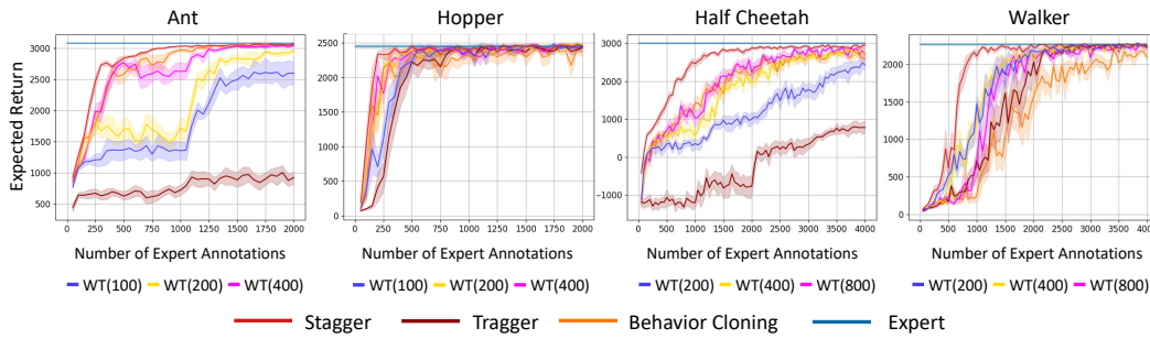
Figure 6: Sample efficiency of algorithms on MuJoCo tasks, showing expected return vs. number of annotations ( C = 1 ). WARM-TRIGGER (WT) is initialized with 1/20, 1/10, or 1/5 of the total annotation budget as offline demonstrations. Specifically, WT( n ) refers to WT with offline demonstrations of total length n . Although the performance of WT improves with more offline demonstrations, both TRIGGER and WARM-TRIGGER remain inferior to STAGGER and, in many cases, even underperform Behavior Cloning, confirming the advantage of state-wise over trajectory-wise annotations.
