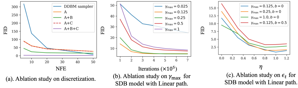
Figure 4: Ablation studies on discretization, \gamma_{\max} and \epsilon_t . (a). We evaluate different discretization schemes on Edges2handbags ( 64 \times 64 ) dataset using DDBM-VP pretrained model, A represents simple Euler discretization in Eq. (13), B represents setting \epsilon_t = 0 for the last 2 steps, C represents using Eq. (12) for \epsilon_t = 0 . (b). Ablation study on \gamma_{\max} evaluated by DIODE ( 64 \times 64 ) dataset. (c). Ablation study on \epsilon_t through our ECSI model with Linear path on Edges2handbags ( 64 \times 64 ) dataset, where \epsilon_t = \eta(\gamma_t \dot{\gamma}_t - \frac{\dot{\alpha}_t}{\alpha_t} \gamma_t^2) .
