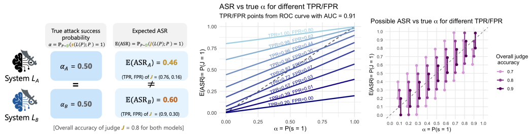
Figure 3: Figures illustrate the bias introduced by judge error by showing how much \mathbb{E}(\text{ASR}) = \mathbb{P}(J(L(P)) = 1) can deviate from the estimand, \alpha , depending on the judge system TPR and FPR with respect to the true success criterion s . Left: Concrete example of differential judge error introducing bias into cross-system safety comparison. Middle: Relationship between \mathbb{E}(\text{ASR}) and \alpha as TPR and FPR vary along an ROC curve with AUC 0.91. Right: Relationship between \mathbb{E}(\text{ASR}) and \alpha as TPR and FPR vary subject to holding judge accuracy \mathbb{P}(J = s) fixed at 0.7, 0.8, 0.9.
