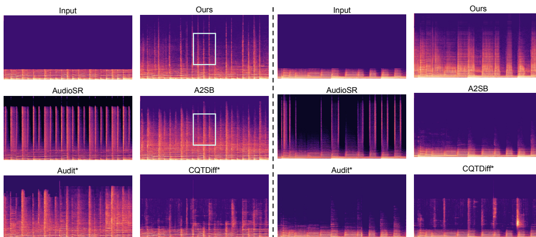
Figure 13: Qualitative comparison from A 2 SB's demo page.
