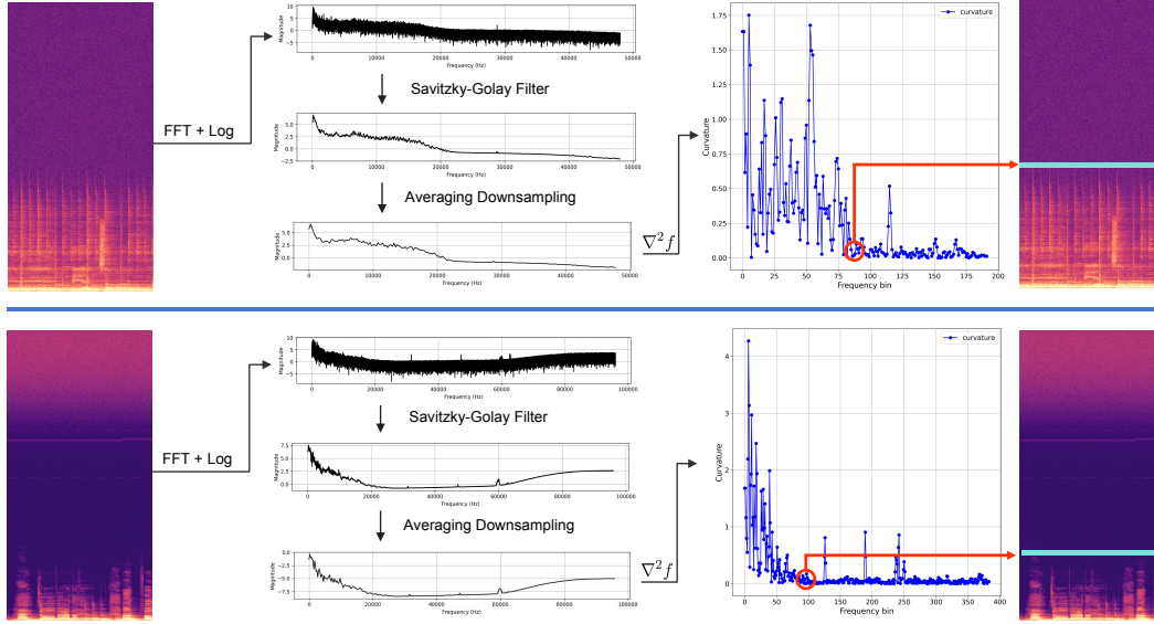
Figure 8: Overview of our proposed curvature-aware estimation pipeline. Given a raw waveform x , we first compute its magnitude spectrum via FFT, followed by Savitzky-Golay smoothing and local downsampling to obtain a denoised spectrum. We then compute the second-order curvature over the log-magnitude spectrum to detect the effective cut-off frequency f_{\text{eff}}(x) , which is used for downstream low-pass filtering. As a result, our method is robust to high-frequency noise.
