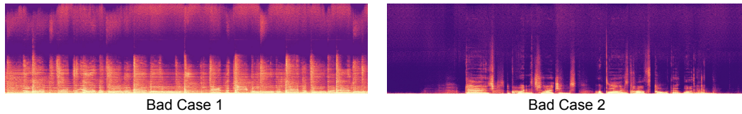
Figure 6: The impact of high-frequency noise on super-resolution outputs. Without an effective choice of f_{\text{target}} , the SR model hallucinates unnatural noise and artifacts in the high-frequency band.
