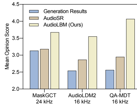
Figure 1: AudioLBM significantly improves the perceptual quality of text-to-speech [111], text-to-audio [63], and text-to-music [53] generation, and outperforms the state-of-the-art any-to-48 kHz SR system AudioSR [62].
