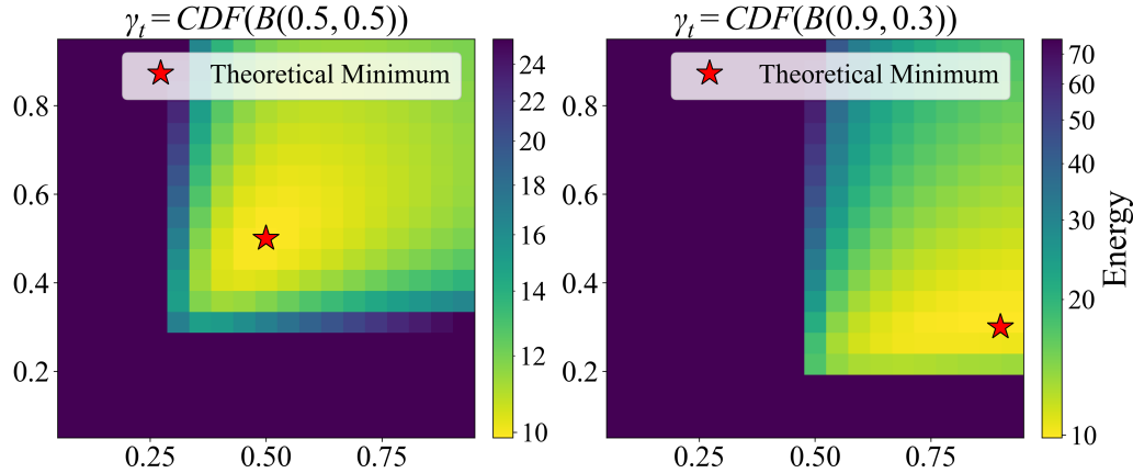
Figure 2: Distinct weight functions \gamma_t shape different energy landscapes and consequently yield different optimal mask schedules \alpha_t^* . Axes represent the beta-parameterization of \alpha_t (see Sec. 3.3). Color intensity indicates energy values from Eq. (14). Red stars mark the theoretical minima under the optimal schedule condition.
