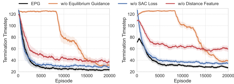
Figure 3: Termination timesteps of pursuer policies under training set (left) and testing set (right)
