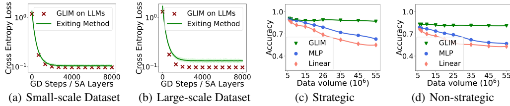
Figure 5: (a) and (b): comparison of cross-entropy losses between ICL and gradient-based methods. (c) and (d): comparison of GLIM with existing models as the data volume continuously increases.
