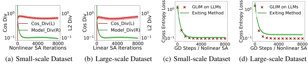
Figure 7: (a) and (b) compare ICL-guided decision rule optimization and gradient-descent methods across data scales; (c) and (d): comparison of cross-entropy losses between ICL and gradient-based methods.
