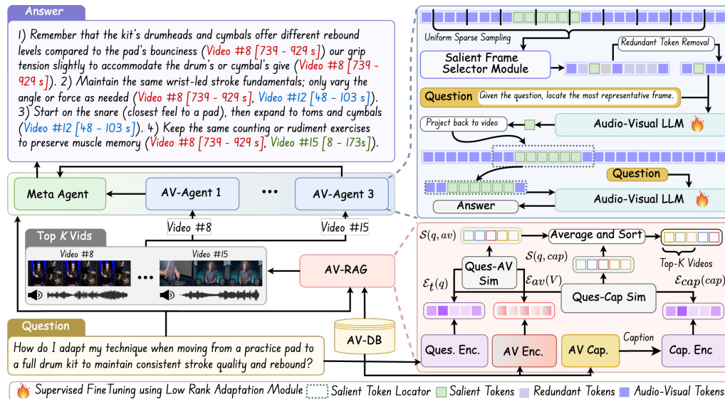
Figure 2: Overview of MAGNET. Given a user query, AV-RAG retrieves the top-K relevant videos (with audio), which are then processed by dynamically spawned Audio-Visual agents and a meta-agent aggregator to generate temporally grounded, step-wise responses. An adaptive, modality-agnostic frame selection module improves performance over baselines (see Tab. 2).
