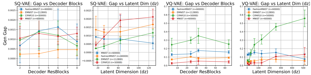
Figure 6: Behavior of the generalization gap when increasing the number of residual blocks of the decoder network and the latent dimension d_z in SQ-VAE (stochastic, left two panels) and VQ-VAE (deterministic, right two panels) models.
