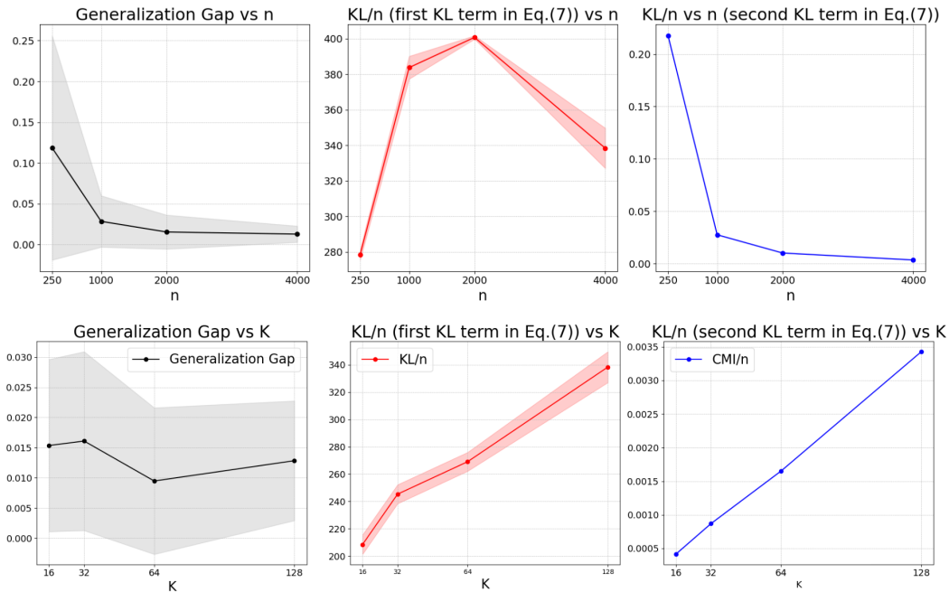
Figure 7: Behavior of the generalization gap and the two KL terms from Eq. (7) on the MNIST dataset ( K = 128, d_z = 64 ). (Top row) Asymptotic behavior as a function of sample size n . (Bottom row) Behavior as a function of codebook size K (for n = 2000 ).
