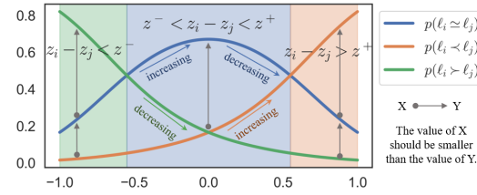
Figure 1: Schematic of probability monotonicity and probability orderliness.
