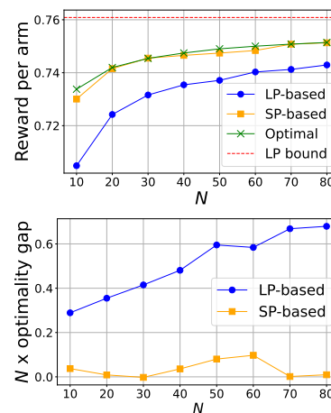
Figure 1: Comparison of LP and SP-based policies.
