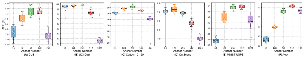
Figure 10: ACC results of AGF-TI with different anchor numbers.
