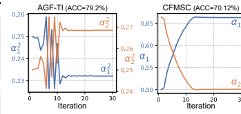
Figure 3: \alpha comparison on CUB.
