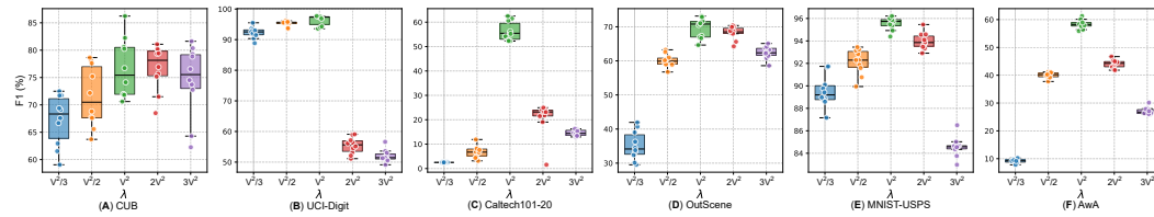
Figure 14: Parameter sensitivity analysis of \lambda in terms of F1.
