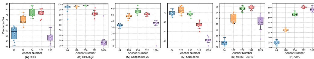
Figure 12: Precision results of AGF-TI with different anchor numbers.
