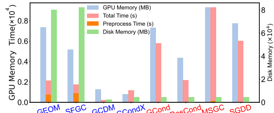
Figure 2: Comparison of GPU memory, disk memory, preprocess time, and total time on Arxiv ( r = 0.5\% ).
