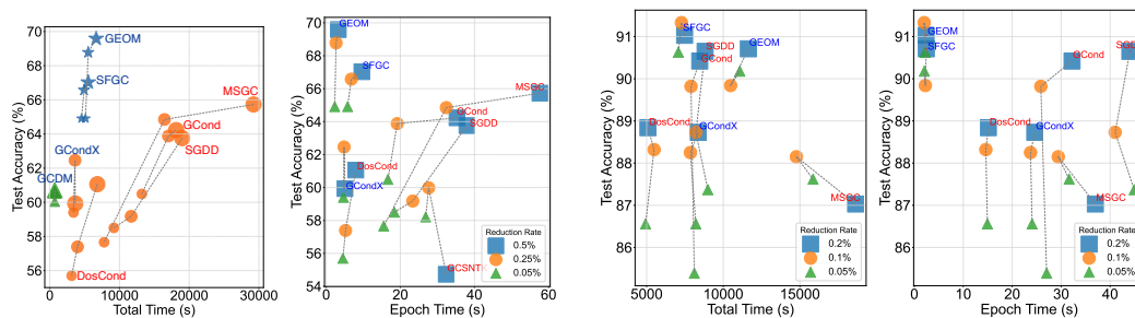
Figure 6: Performance vs. Total Time and Epoch Time on Arxiv (left two) and Reddit (right two).
