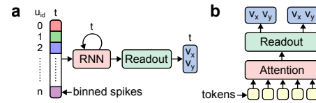
Figure 1: Existing deep learning models for neural decoding. (a) Recurrent neural networks (RNNs). (b) Attention-based models such as Transformers.
