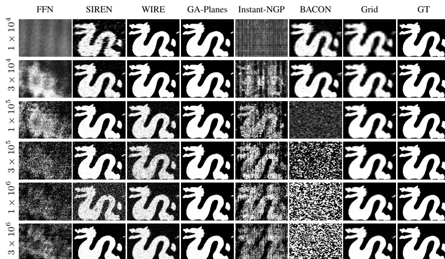
Figure 23: 3D Dragon Occupancy Super-Resolution. SIREN, WIRE, GA-Planes, and Grid all produce reasonable results, with GA-Planes' the most consistent across model sizes. BACON struggles to represent the shape at large model sizes. Detailed quantitative results are in Table 25.
