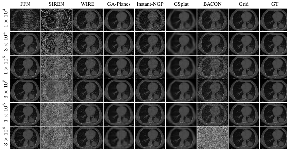
Figure 18: CT Reconstruction. All models except SIREN and BACON successfully reconstruct the CT image at medium to large model sizes. However, the qualitative performance of GA-Planes degrades in the over-parameterized regime, perhaps due to lack of explicit regularization for this underdetermined inverse problem. No model outperforms the TV-regularized Grid at any model size in the compressive regime. Detailed quantitative results are in Tables 22 to 24.
