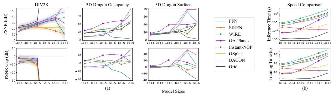
Figure 4: Overfitting Capacity and Computational Efficiency. (a) Overfitting capacity of different models evaluated on the 2D DIV2K and 3D Stanford Dragon datasets. PSNR trends indicate how well each model fits the training data as a function of model size (top) as well as relative performance compared to the Grid baseline (bottom). (b) Computational efficiency analysis, showing inference and training times for each model. While WIRE achieves superior overfitting capacity in some cases, it requires significantly more computation time—approximately 10\times that of the next slowest model.
