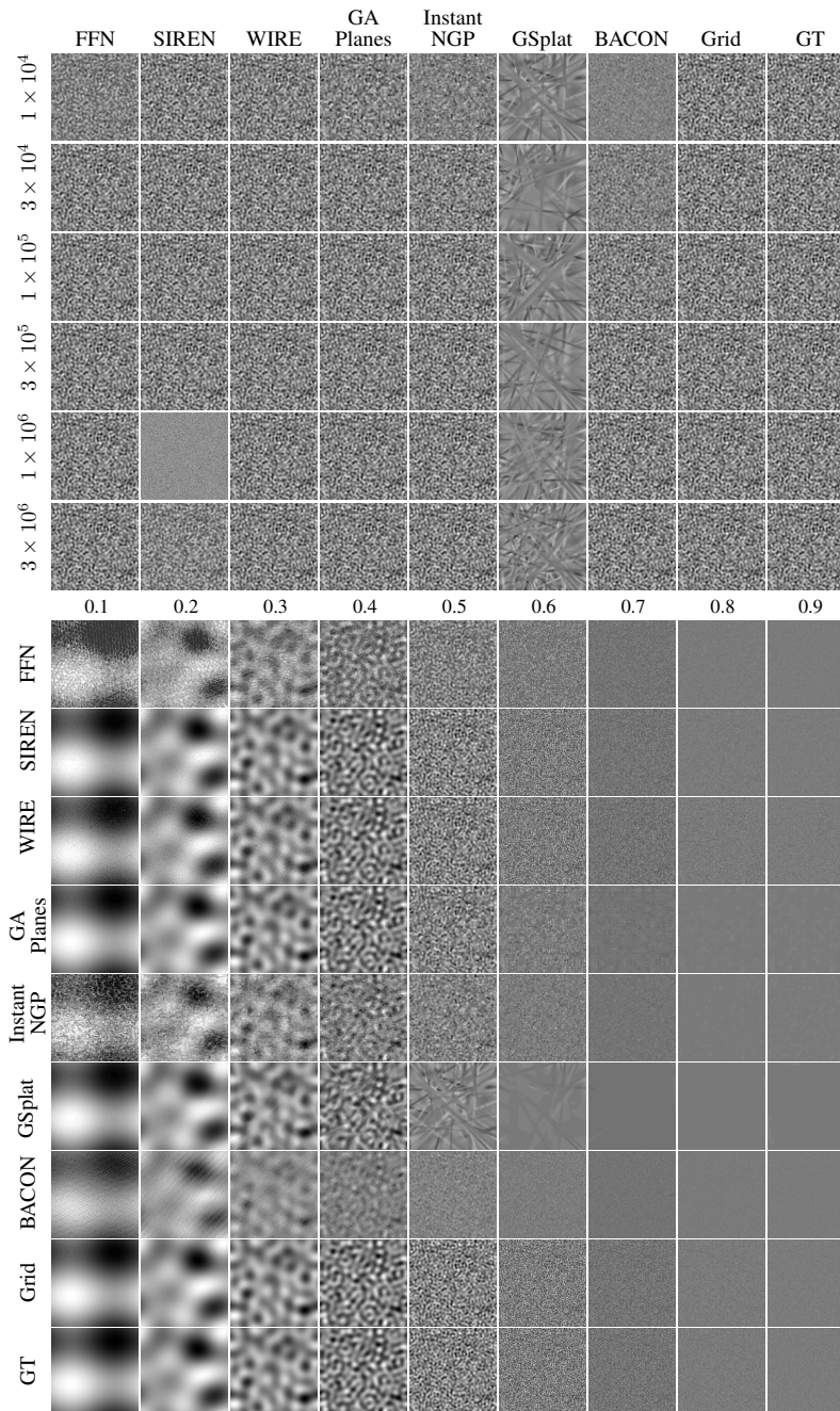
Figure 8: 2D Bandlimited Signal overfitting with bandwidth = 0.5 (top) and model size = 1 \times 10^4 (bottom). Sinusoid-based models (FFN, SIREN) and BACON which is also bandlimited exhibit characteristic wave-like artifacts, while GA-Planes introduces subtle blurring and axis-aligned artifacts. Instant-NGP struggles with severe noise, likely due to hash collisions. Grid remains stable under limited resource conditions but blurs high-bandwidth signals that exceed the Nyquist frequency. Detailed quantitative results are in Tables 8 to 10.
