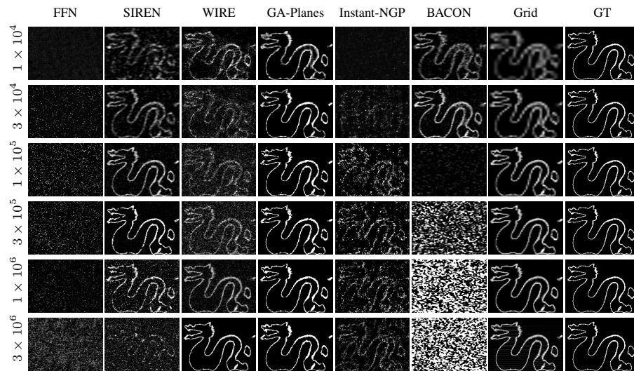
Figure 24: 3D Dragon Surface Super-Resolution. For 3D super-resolution, only SIREN, WIRE, GA-Planes, BACON, and Grid successfully capture surface details at some model sizes. GA-Planes consistently achieves high-quality results across model sizes, while WIRE and Grid struggle in under-parameterized conditions and SIREN and BACON show nonmonotonic performance with model size. Detailed quantitative results are in Table 25.
