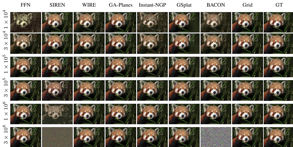
Figure 13: DIV2K Overfitting. FFN and Instant-NGP struggle to overfit colors with small model sizes. Similar to synthetic signals, SIREN and BACON exhibit noisy artifacts and BACON exhibits unstable performance in the over-parameterized regime. Detailed quantitative results are in Tables 20 and 21.
