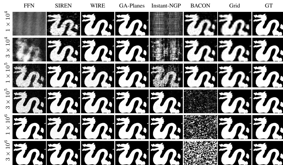
Figure 14: 3D Dragon Occupancy Overfitting. All models except BACON effectively learn the signal when model size matches or exceeds the inherent signal size of 1 \times 10^6 . At small model sizes (high compression), WIRE and GA-Planes produce much sharper representations than the Grid, which is blurry when underparameterized. Detailed quantitative results are in Table 20.
