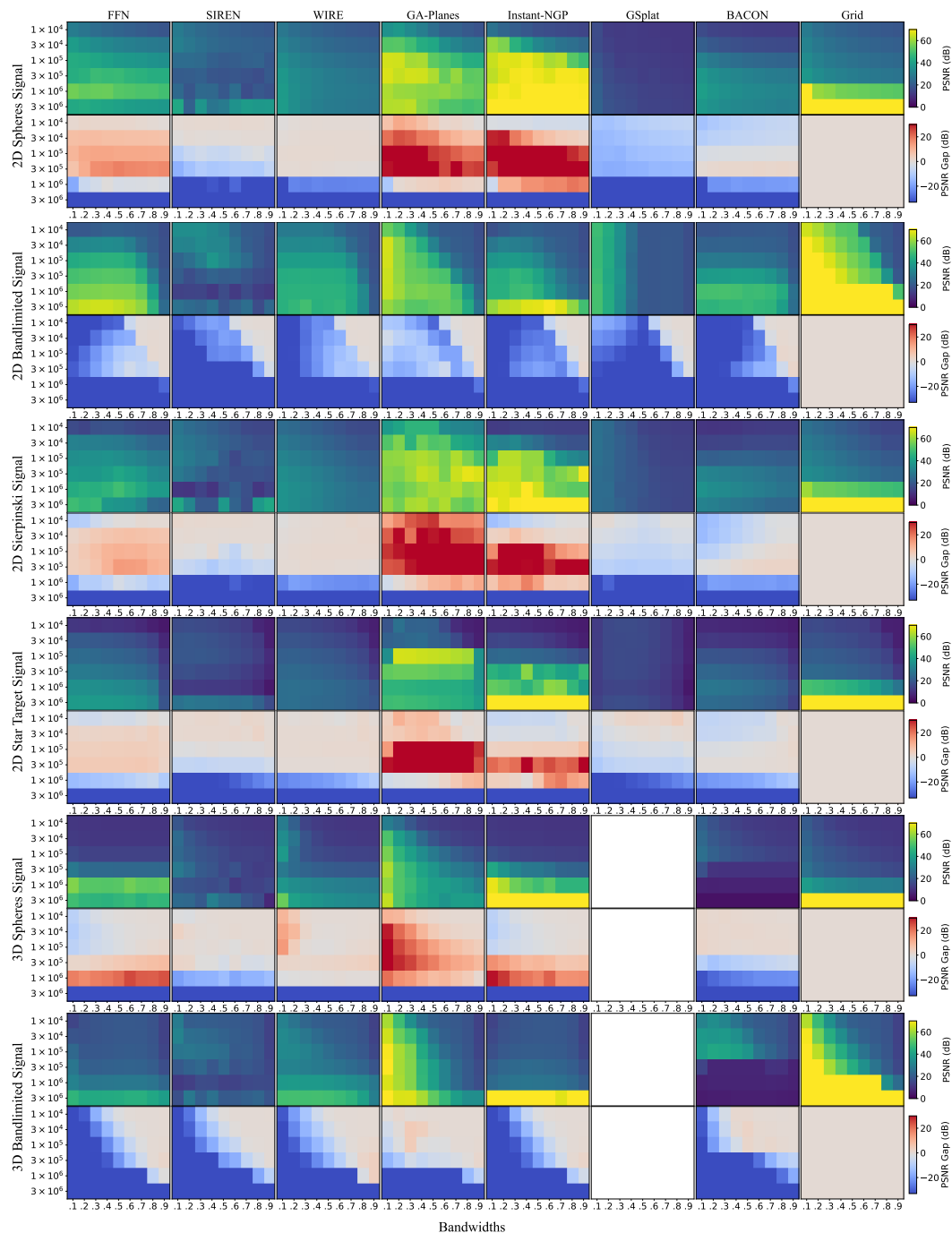
Figure 3: Overfitting Synthetic Signals: INR and INR - Grid Heatmaps. Red indicates regimes where other models outperform the Grid baseline; blue indicates regimes dominated by the Grid baseline. Each first row shows absolute PSNR values, while each second row shows the PSNR gap relative to the Grid baseline (i.e., PSNR - Grid PSNR). See Section 3.1 for in-depth discussion.
