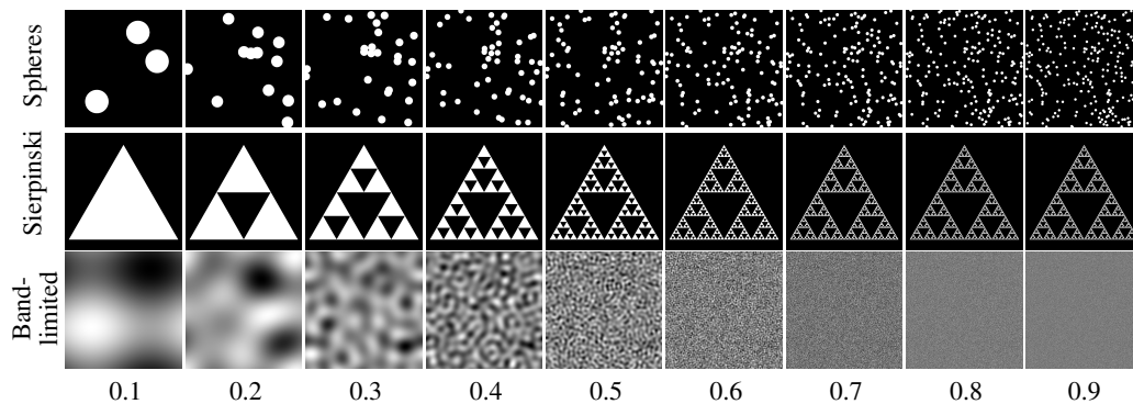
Figure 1: Synthetic Signals. Rows represent synthetic signal types, and columns represent effective bandwidths from 0.1 to 0.9. Signal detail and complexity increase with effective bandwidth.
