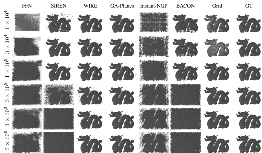
Figure 25: 3D Dragon Occupancy Super Resolution Render. Detailed quantitative results are in Table 25.
