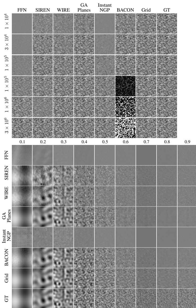
Figure 12: 3D Bandlimited overfitting with bandwidth = 0.5 (top) and model size = 1 \times 10^4 (bottom). FFN, Instant-NGP, and BACON show similar behavior as on the 3D Spheres, while other models exhibit similar behavior as with 2D Bandlimited images. Detailed quantitative results are in Table 19.
