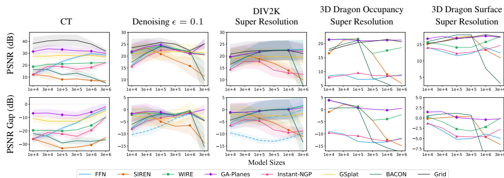
Figure 6: Quantitative Generalization and Inverse Problems Results. PSNR vs. model size trends indicate how well each model performs each generalization task as a function of model size (top) as well as relative performance compared to the TV-regularized Grid baseline (bottom). WIRE and GA-Planes perform best at highly compressed 3D super-resolution, but the simple Grid baseline generally outperforms other signal representation methods across these tasks.
