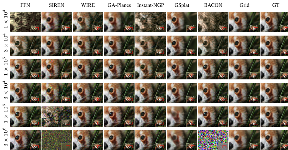
Figure 20: DIV2K Denoising , \epsilon = 0.05 . WIRE and GA-Planes produce sharper reconstructions but exhibit characteristic noisy and grid-like artifacts, respectively, at the smallest model size. SIREN and Grid produce reasonable but characteristically blurry results in the underparameterized regime, and SIREN and BACON exhibit unstable performance when overparameterized. Instant-NGP and FFN also perform well at denoising, except under the strongest compression. GSplat produces sharp details in some regions but misses details in others. Detailed quantitative results are in Tables 22 to 24.
