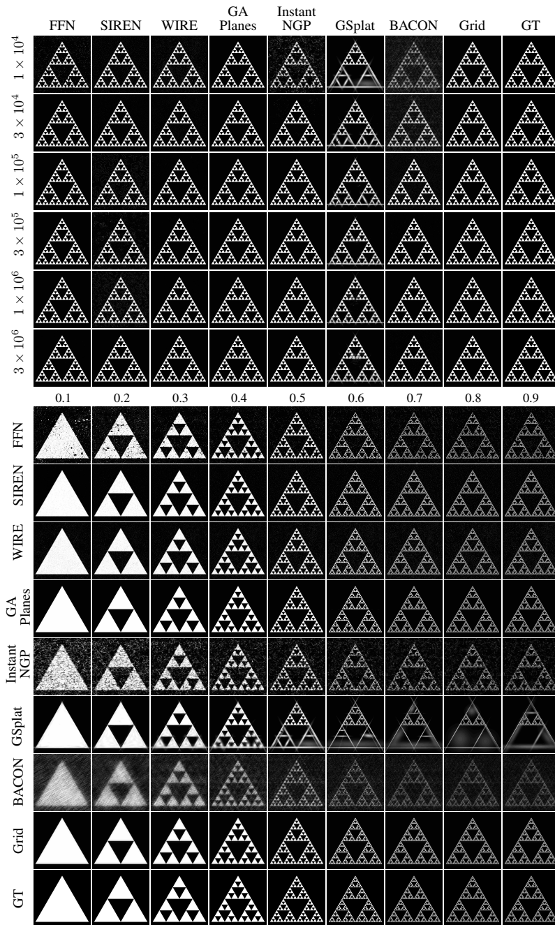
Figure 9: 2D Sierpinski overfitting with bandwidth = 0.5 (top) and model size = 1 \times 10^4 (bottom). In general, performance improves as model size increases. We note that for some signals including Sierpinski, Instant-NGP and BACON produce noisy outputs and GSplat fails to fit high frequency regions. Detailed quantitative results are in Tables 11 to 13.
