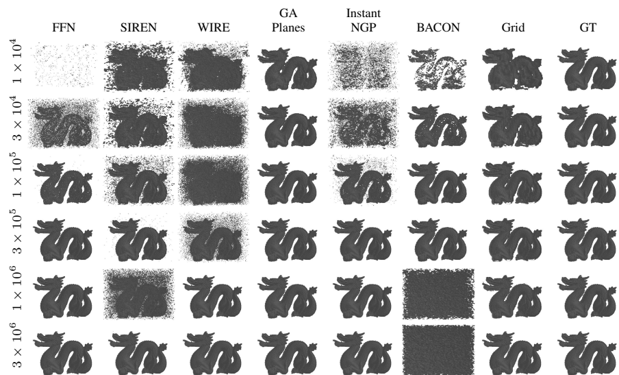
Figure 17: 3D Dragon Surface Overfitting Render. For most models, results parallel results at dragon occupancy fitting. However, WIRE and BACON notably exhibit different performance in these two tasks, both struggling to fit the dragon surface at small model sizes. Detailed quantitative results are in Table 20.
