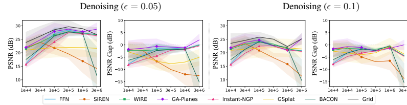
Figure 19: Denoising Evaluation. Denoising performance of various models on the DIV2K dataset, evaluated using 10 images. Grid with TV regularization consistently outperforms other methods at both noise levels.
