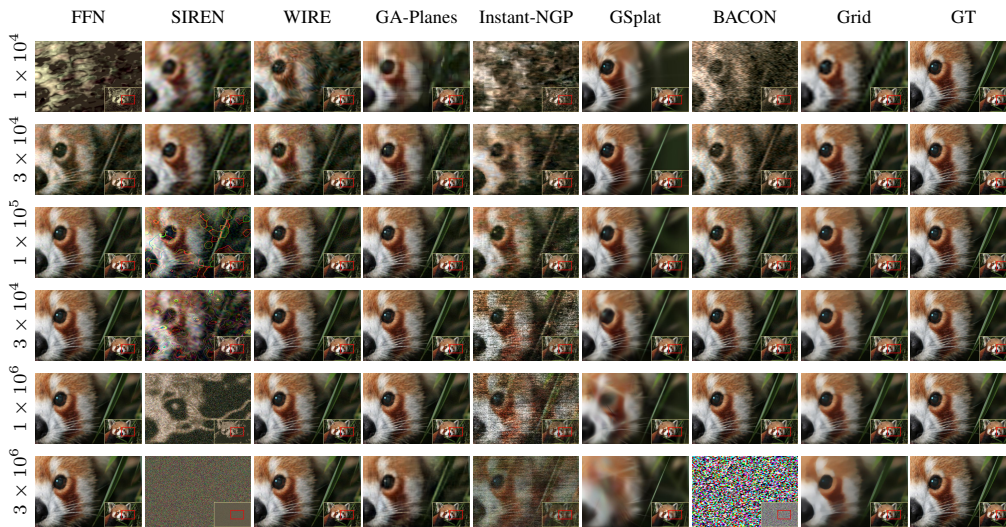
Figure 22: DIV2K Super-Resolution. All methods except Instant-NGP perform reasonably well at super-resolution, though only SIREN, WIRE, GA-Planes, GSplat, and Grid perform well under extreme compression. Detailed quantitative results are in Tables 22 to 24.
