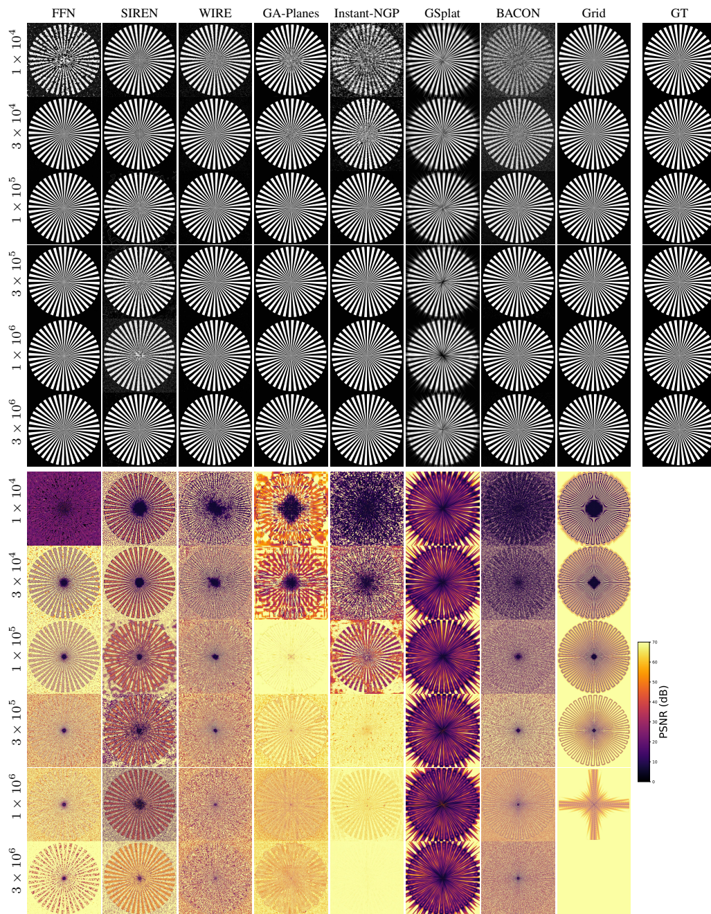
Figure 10: 2D Star Target overfitting outputs (top) and error maps (bottom). As the signal transitions to higher frequencies toward the center of the Star Target, most models incur larger reconstruction errors (visualized in the lower figure via pixelwise PSNR). The error maps visually reveal the implicit biases of each model, illustrating which regions (e.g., background, constant regions, edges) are best captured by each model at each level of compression. Detailed quantitative results are in Tables 14 to 16.
