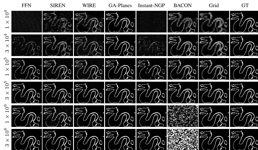
Figure 15: 3D Dragon Surface Overfitting. Results mirror those for the solid 3D Dragon occupancy overfitting task. At small model sizes, GA-Planes produces the sharpest representation. Detailed quantitative results are in Table 20.
