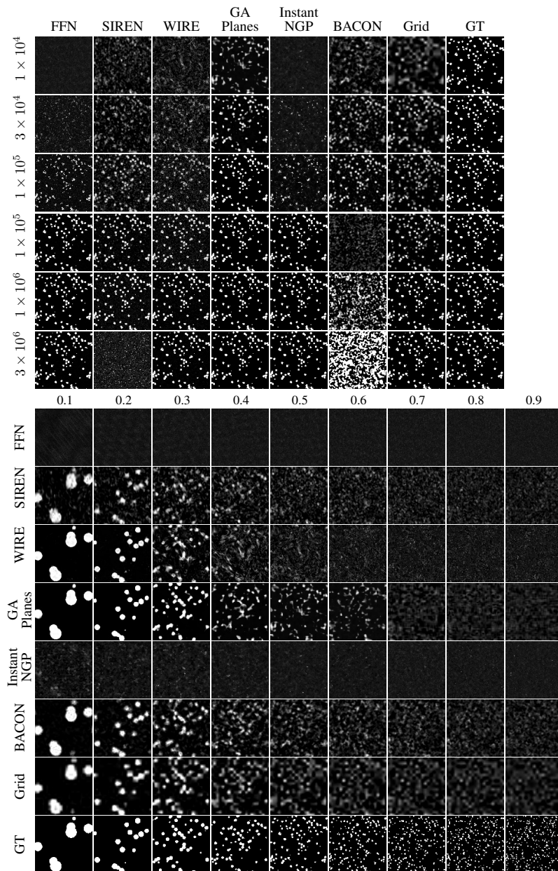
Figure 11: 3D Spheres overfitting with bandwidth = 0.5 (top) and model size = 1 \times 10^4 (bottom). FFN and Instant-NGP struggle to fit the 3D Spheres in the most compressed settings, while BACON suffers instability at large model sizes. Detailed quantitative results are in Tables 17 and 18.
