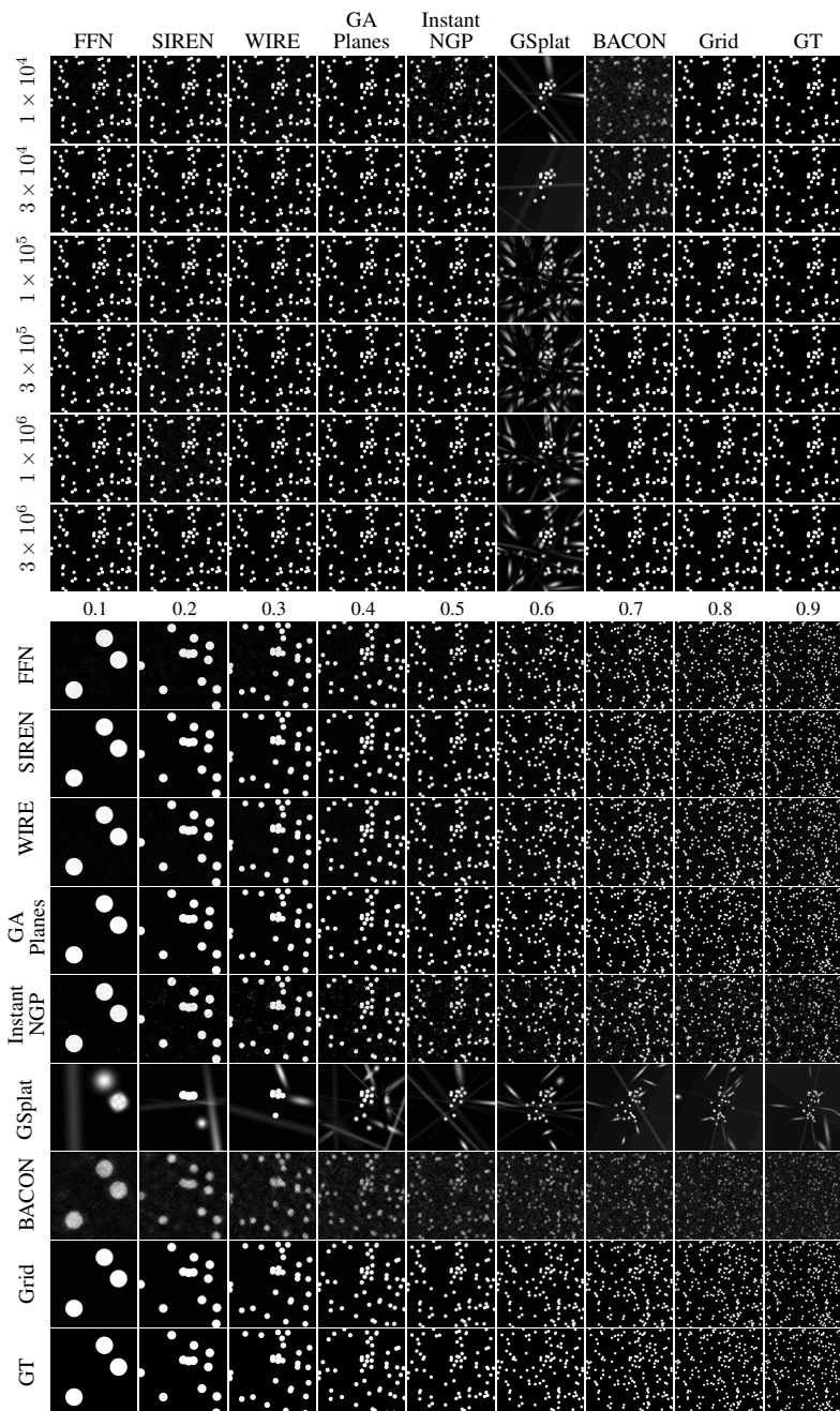
Figure 7: 2D Spheres overfitting with bandwidth = 0.5 (top) and model size = 1 \times 10^4 (bottom). For the 2D Spheres signal, most models effectively capture the structure even in highly compressed settings. However, GSplat struggles to fit some regions of the image and BACON produces a blurry representation at small model sizes. Detailed quantitative results are in Tables 5 to 7.
