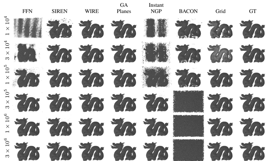
Figure 16: 3D Dragon Occupancy Overfitting Render. Detailed quantitative results are in Table 20.
