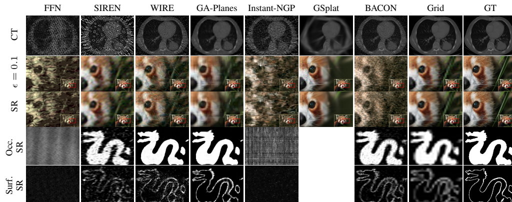
Figure 5: Qualitative Generalization and Inverse Problems Results. In CT reconstruction, Grid with TV regularization achieves the best results. Experiments on the DIV2K dataset are zoomed in to highlight image details. For image denoising and super-resolution, WIRE produces sharp images but introduces texture artifacts. GA-Planes outperforms other methods in volume and surface super-resolution. Artifacts in each model’s output throughout the inverse problem tasks reveal their inherent structural biases (e.g., sinusoidal artifacts in FFNs and SIREN, line artifacts in GA-Planes).
