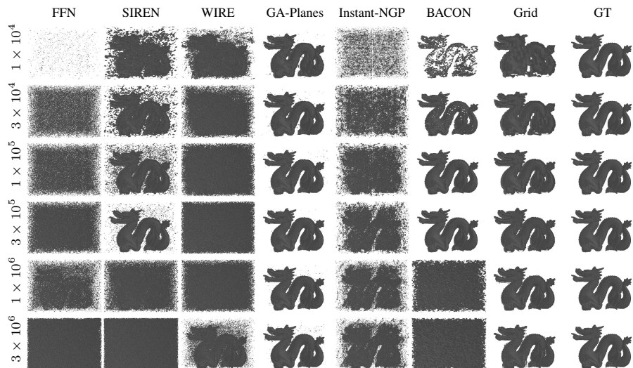
Figure 26: 3D Dragon Surface Super Resolution Render. Detailed quantitative results are in Table 25.
