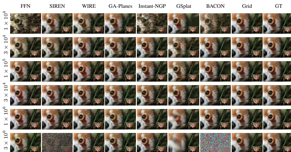
Figure 21: DIV2K Denoising , \epsilon = 0.1 . The overall trends remain similar to the \epsilon = 0.05 case, but due to the increased noise level, all models struggle to effectively remove noise in the reconstructed outputs. Detailed quantitative results are in Tables 22 to 24.
