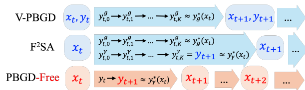
Figure 1: Update schemes for V-PBGD, F 2 SA and PBGD-Free. V-PBGD [78] ( top ) and F 2 SA [45] ( middle ) refine the LL variable over multiple steps before updating x_t via \nabla_x \tilde{F}_\gamma(x_t, y_t) for V-PBGD or \nabla_x \tilde{F}_\gamma(x_t, y_t) for F 2 SA while PBGD-Free ( bottom ) applies a 1-step inner update to find a more efficient yet potentially less accurate \nabla_x f(x_t, y_{t+1}) \approx \nabla F_\gamma(x_t) .
