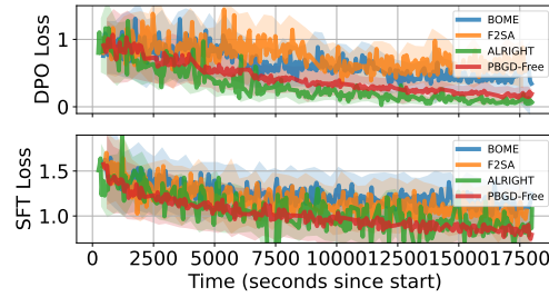
Figure 7: Train losses vs. time for different algorithms in solving (3) (or bi-objective learning for ALRIGHT) on LLAMA-3-3B [31].
