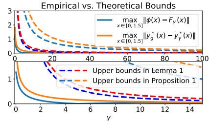
Figure 4: Empirical bounds for \|\phi(x) - F_\gamma(x)\| and \|y_\gamma^*(x) - y_g^*(x)\| versus the theoretical upper bounds in Proposition 1 and Lemma 1 for the illustration of representation learning PEFT (3). The lower plot shows a smaller scale.
