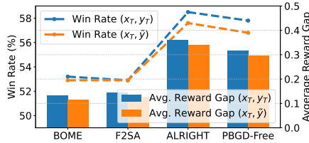
Figure 11: Average Reward Gap (↑) and Win Rate (↑) for different algorithms for PEFT LLAMA-3-3B on [31] with the output (x_T, y_T) via each method in S1 and the outcome (x_T, \hat{y}) from post-SFT-tuning on another dataset with fixed-backbone in S2 ).
