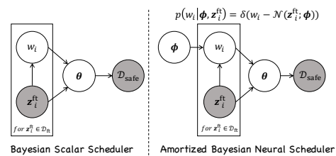
Figure 2: Graphical models for the Bayesian Scalar Scheduler (see Sec. 4.2) and Amortized Bayesian Neural Scheduler (see Sec. 4.3).
