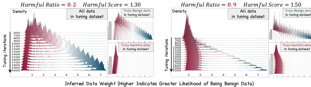
Figure 1: For encountered datasets with unknown and different harmful ratios, BDS adaptively schedules data into higher and lower weight groups during tuning ( largest panels ). To verify correctness of our data scheduling, we observe that most truly benign data indeed receive higher weights ( top right panels ), while almost all truly harmful data consistently receive lower weights ( bottom right panels ).
