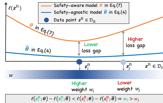
Figure 4: Intuition behind weight update in Eq. (8).
