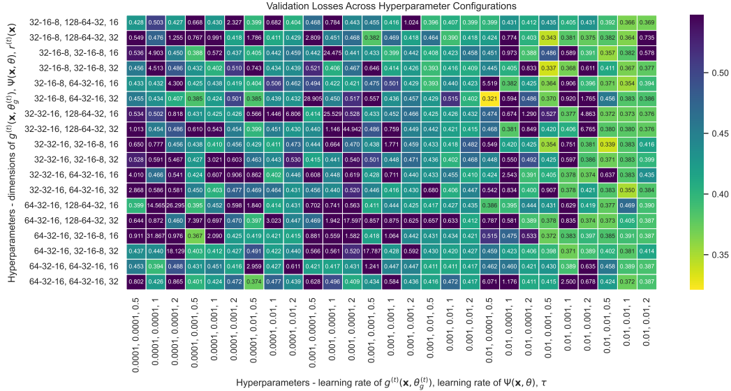
Figure 8: Hyperparameter sensitivity study results of our proposed bi-level knowledge distillation approach on the AKI dataset.
