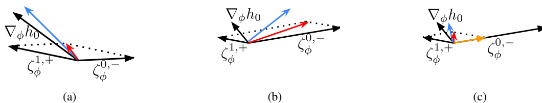
Figure 12: Illustration of the gradient scaling with two levels. The coloured arrows indicate gradient of the correction term (red), total gradient (blue), and scaled gradient (orange) respectively. (a) Ideal case: \|\nabla_\phi h_c(\phi)\| remains small and works as a correction to \nabla_\phi h_0(\phi) . (b) In the later stage of training, \nabla_\phi h_0(\phi) and \zeta_\phi^{1,+} diminishes and \zeta_\phi^{0,-} starts to dominate the optimisation. (c) Gradient scale adjustment: We scale \zeta_\phi^{0,-} such that \|\zeta_\phi^{1,+}\| \approx \|\zeta_\phi^{0,-}\| and \|\nabla_\phi h_c(\phi)\| remains small throughout the training as intended.
