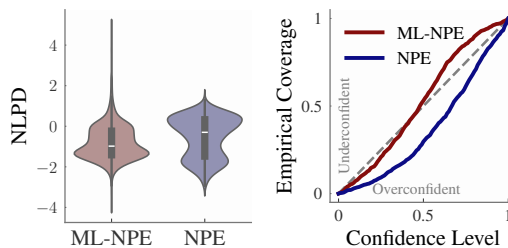
Figure 5: NLPD \downarrow and empirical coverage of NPE and ML-NPE for the cosmological inference task.
