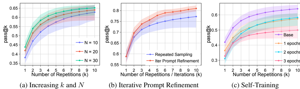
Figure 12: InterCode CTF (Test) performance of Gemma3-12B-It model under NYU CTF agent scaffolding with different degrees of freedom. While some degrees of freedom (like self-training) do not show positive signals in our search space, repeated sampling, increasing max rounds of interactions, and iterative prompt refinement can still substantially improve agent’s performance.
