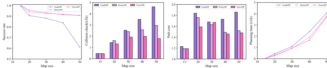
Figure 9: Performance comparison of NeuroMP, BrainyMP and GraphMP under different map sizes environments. (a) Success rate, (b) Collision check, (c) Path cost, (d) Planning time.
