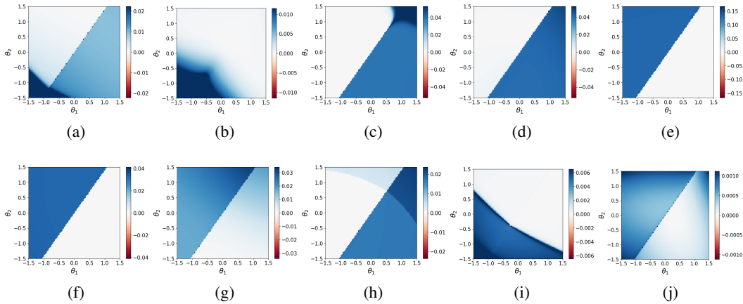
Figure 11: Loss after training student network for 100 steps. We rescale the \pi_3 \rightarrow \pi_3 map as \sqrt{n-1}\theta_1 I + \theta_2(\mathbf{11}^T - I) .
