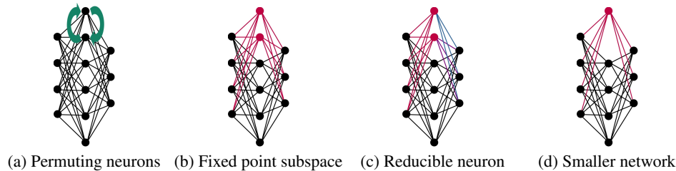
Figure 2: (a) Subgroup of global parameter symmetry which permutes two neurons. (b) Corresponding fixed point subspace where both input and output weights of these two neurons are the same. (c) There is an additional local parameter symmetry on the output weights. In particular, as long as the sum of output weights of the neurons is the same, we compute the same function. (d) Smaller network with one fewer neuron computing the same function.
