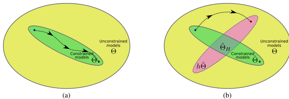
Figure 1: (a) Standard viewpoint of why constraints may help. If we know the ground truth function satisfies some type of constraint, then enforcing such constraints may reduce the search space allowing for better training. (b) In reality, unconstrained networks contain many parameter symmetries. However, enforcing constraints (such as equivariance) require choices that breaks some of these symmetries. These broken symmetries are "hidden" to the constrained model but still influence gradient values and in some cases create spurious minima and hinder learning. Further, we empirically observe that when completely relaxing equivariance constraints, a network can sometimes "jump" between subspaces corresponding to different ways of enforcing the same type of constraint.
