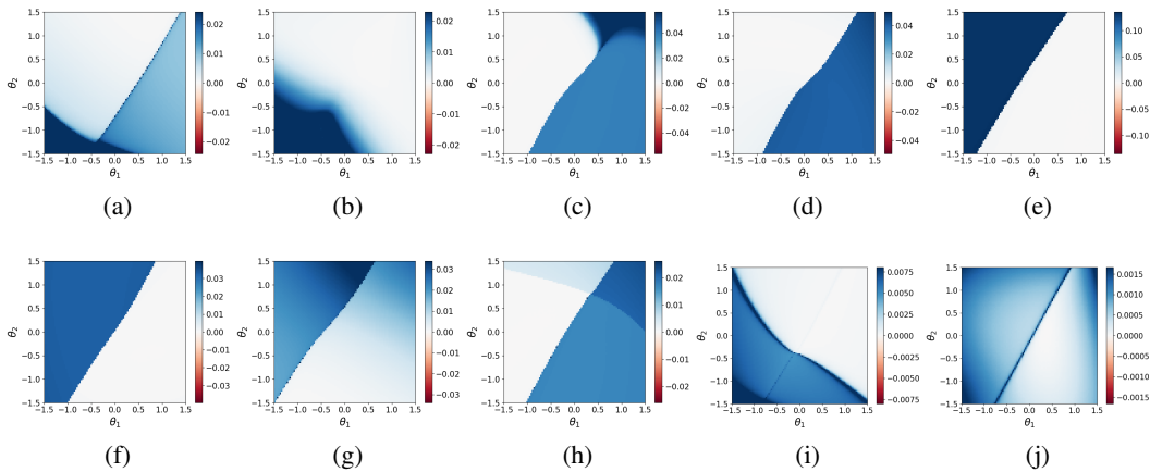
Figure 10: Loss after training student network for 100 steps. We directly parameterize the \pi_3 \rightarrow \pi_3 map as \theta_1 I + \theta_2 (\mathbf{11}^T - I) .
