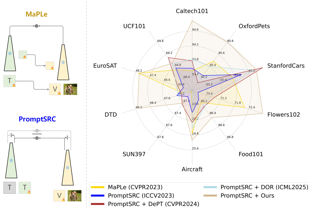
Figure 1: Performance comparison of Ours with prompting plug-in methods under the cross-dataset generalization. For cross-dataset generalization, the MaPLE (without visual loss) is higher than PromptSRC (with visual loss), as shown in Table 1. To improve the cross-dataset generalization of PromptSRC (with visual loss), we propose a plug-in design, improving the performance, surpassing the plug-and-play DePT [29] (CVPR2024) and DOR [30] (ICML2025). The green ‘T’ and yellow ‘V’ represent learnable textual prompts and visual prompts, respectively.
