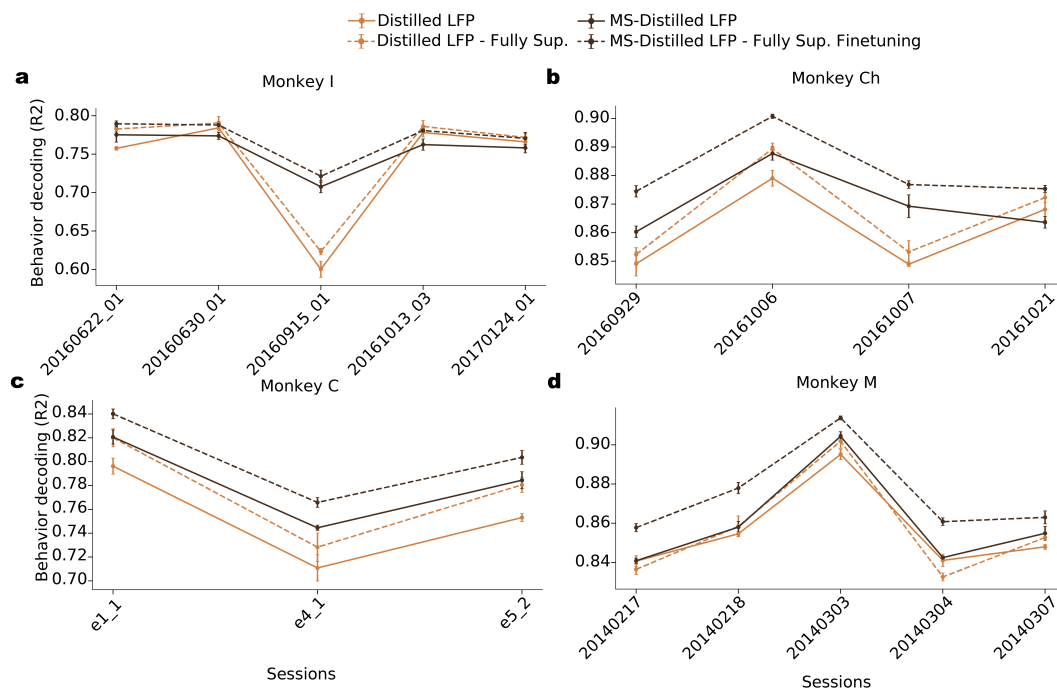
Figure 17: Behavior decoding performances ( R^2 ) of fully-supervised MS-Distilled LFP and Distilled LFP models. Both models were trained (and then fine-tuned for the MS-Distilled LFP model) through the supervised distillation objective in Eq. 3, and the teacher MS-Spike models were fine-tuned also in a fully-supervised manner.
