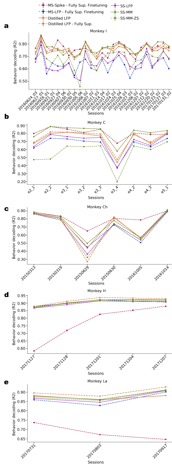
Figure 14: Behavior decoding performances ( R^2 ) in fully-supervised (Fully Sup.) setting on the recording sessions that were used in pretraining of MS-Spike and MS-LFP models. Each panel (a-e) shows decoding results across sessions for individual monkeys (Monkeys I, C with LFP signals, and Monkeys Ch, H, and La with LFP power signals). Unlike Fig. 12, we demonstrate MS-Spike and MS-LFP models that are fine-tuned in a fully-supervised manner just with the behavior regression objective, and Distilled LFP models that are trained via the supervised distillation objective in Eq. 3 with fully-supervised MS-Spike models being teachers. Single-session models are trained only through the behavior regression objective, as done for Figs. 6, 12, 13.
