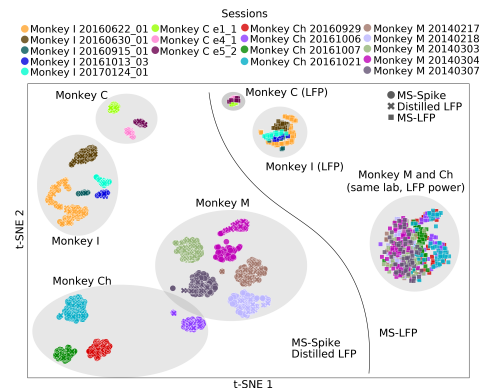
Figure 4: t-SNE representations of time-averaged latent representations across MS-Spike, MS-LFP, and Distilled LFP models across recording sessions from 4 subjects held-out for fine-tuning.
