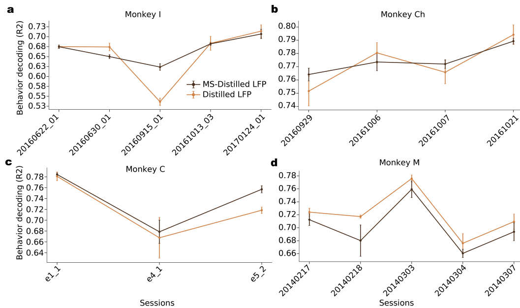
Figure 15: Behavior decoding performances ( R^2 ) of unsupervised MS-Distilled LFP and Distilled LFP models. Both models were trained (and then fine-tuned for the MS-Distilled LFP model) through the unsupervised distillation objective in Eq. 1, where teacher MS-Spike models were fine-tuned also in an unsupervised manner.
