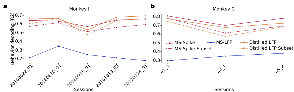
Figure 9: Behavior decoding performances ( R^2 ) of the subset MS-Spike model and Distilled LFP models by using the fine-tuned subset MS-Spike models as the teachers. Performance averages are computed across all held-out fine-tuning sessions of the denoted monkeys (same sessions as in Fig. 3).
