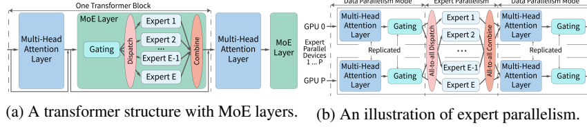
Figure 1: An example of a transformer block with MoE layer and expert parallelism.
