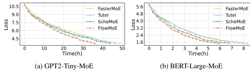
Figure A.2: Loss with time for training GPT2-Tiny-MoE and BERT-Large-MoE.
