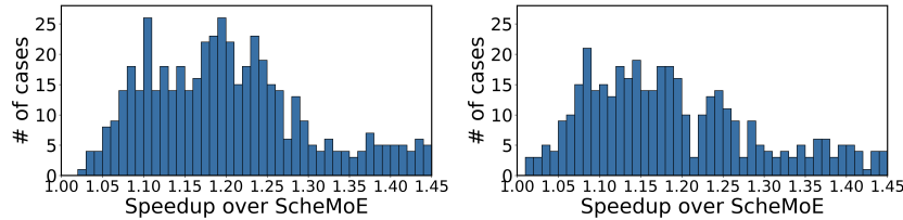
(a) Speedup on Cluster 1.
