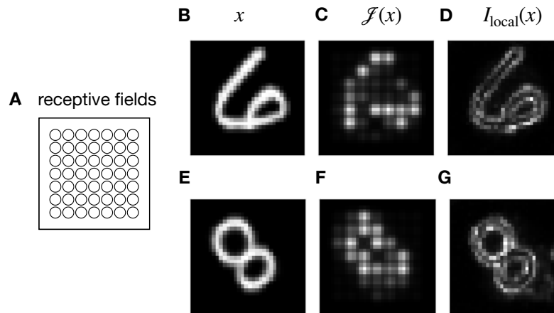
Figure 4: Pixel-wise information decomposition with MNIST stimuli. (A) Simulated population of linear–nonlinear–Poisson (LNP) neurons with circular receptive fields arranged in a grid. (B) Presented visual stimulus. (C) Diagonal of the Fisher information, given by a weighted sum of neural receptive fields. (D) Pixel-wise decomposition of mutual information, I_{\text{local}}(x) . E–G Same as panels A–B, but for a different stimulus.
