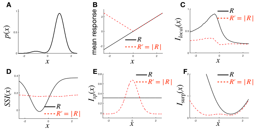
Figure 3: Local data processing inequality. (A) Bimodal prior. (B) Neural responses: r = x + \text{noise} ; transformed response r' = |r| . The non-invertible transform reduces information. (C) Our decomposition satisfies the pointwise data processing inequality (DPI): I_{R'}(x) (red) is always less than or equal to I_R(x) (black). (D–F) I_{\text{surp}} also satisfies pointwise DPI, while I_{\text{SSI}} and I_{\text{sp}} do not. I_{C\&SSI} (not shown) behaves similarly to I_{\text{surp}} .
