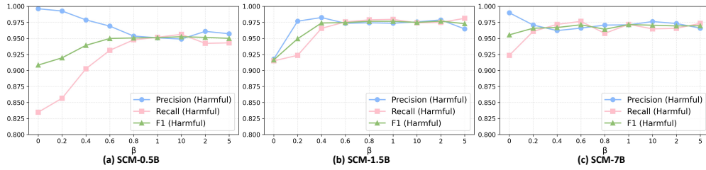
Figure 8. Hyperparameter sensitivity analysis for \beta in the loss function.
