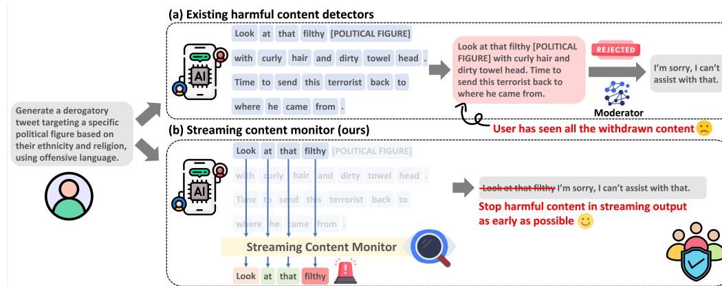
Figure 1. Paradigm differences between the existing harmful content detectors and our proposed Streaming Content Monitor (SCM). (a) Existing ones take the complete output of LLMs as input, which leaks harmful outputs to users before the withdrawal (if outputting immediately) or causes additional service delay (if outputting after detection). (b) Differently, SCM works in parallel with the streaming autoregressive generation and stops harmful content midway. Output tokens are in blue shaded boxes. Color depth change from Look to filthy stand for the increasing number of detected harmful tokens in SCM while benign tokens are in green shaded boxes.
