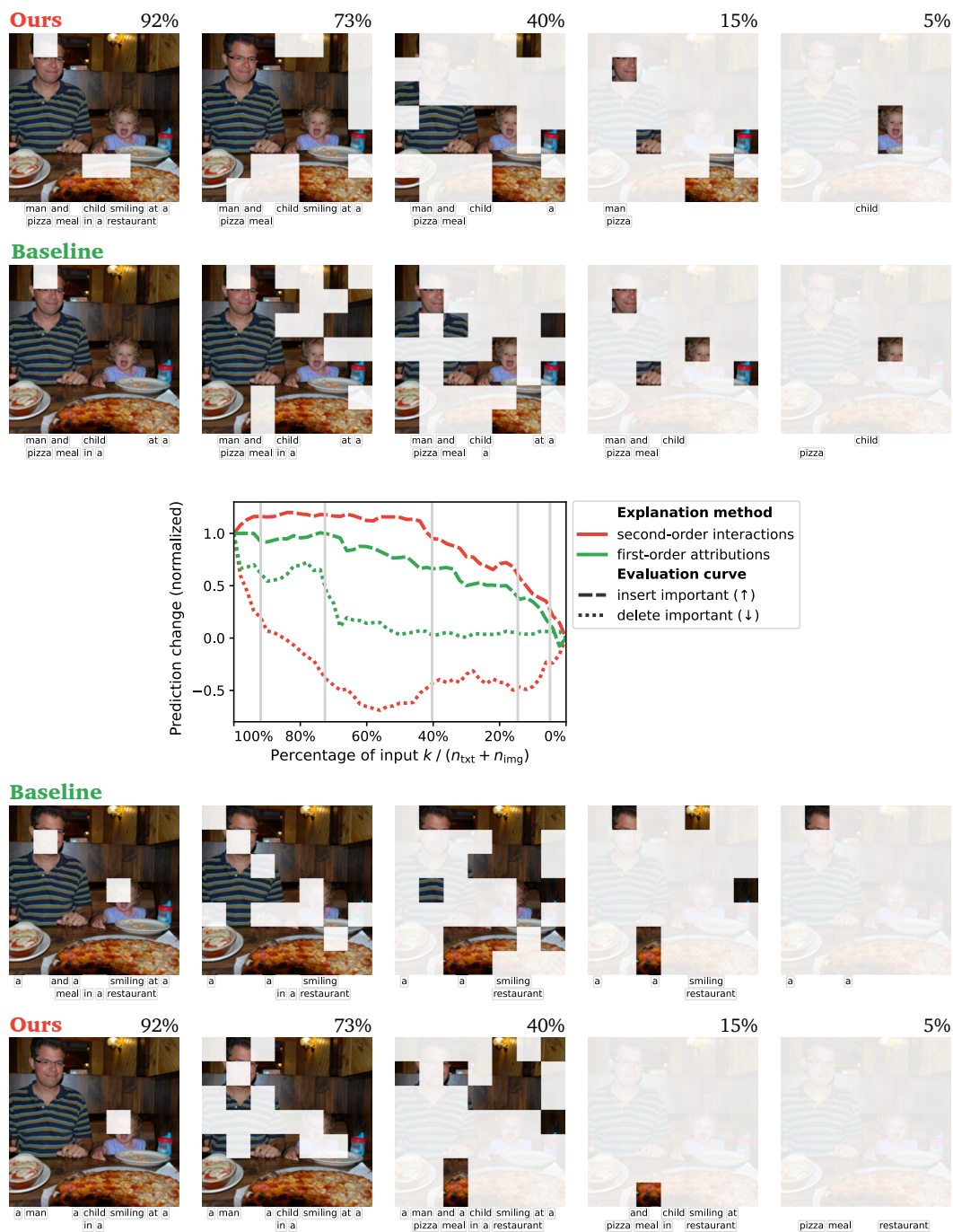
Figure 9: Exemplary insertion/deletion curves for two explanations e computed with FIXLIP and another first-order method. We show five subset visualizations per curve per method. In the case of the baseline method, each consecutive subset needs to include the preceding one, which is not the case for FIXLIP, capturing the complex cross-modal and intra-modal interactions. For example, a child with the corresponding face patches ( top right corner ) gets overvalued by the man–pizza tokens appearing jointly with the corresponding image part (child disappears). Similarly, in the deletion curve, the subsets of text and image tokens interchange with each other at around 50% ( bottom row ).
