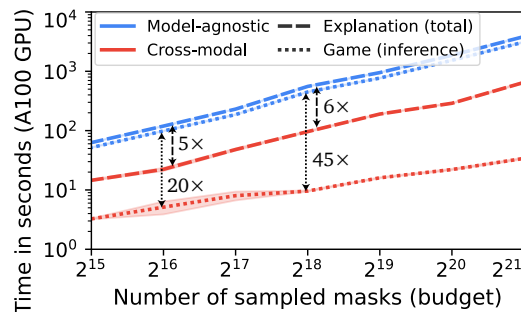
Figure 5: Computation time vs. budget for the FixLIP explanation of SigLIP-2 (ViT-B/32), including game evaluations (model inference).
