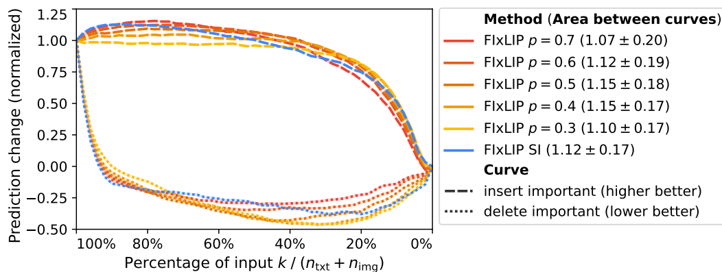
Figure 11: Insertion/deletion curves for SigLIP-2 (ViT-B/32) on MS COCO. Extended Figure 3. AID score (higher is better) for a model-agnostic estimator of FIXLIP with different masking weights. The y-axis is normalized between the model's prediction on the original input (100%) and the fully removed one (0%), where negative values denote that the model is predicting the inputs are unsimilar. We observe a gradual relationship between p and the steepness of the curves at a particular fraction of input deleted. We omit comparison with other baselines in this case as they were originally implemented for CLIP and not SigLIP.
