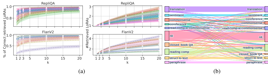
Figure 5: (a) LoRA retrieval performance in RepliQA and FlanV2 for different top-k. Left: % of queries per field for which the correct LoRA \in the set of retrieved LoRAs. Right: # retrieved LoRAs. (b) Retrieval of FlanV2 target domains (left) and corresponding retrieved domains (right).
