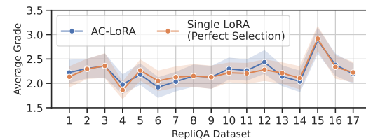
(a) AC-LoRA inference grades w.r.t to single LoRAs.
