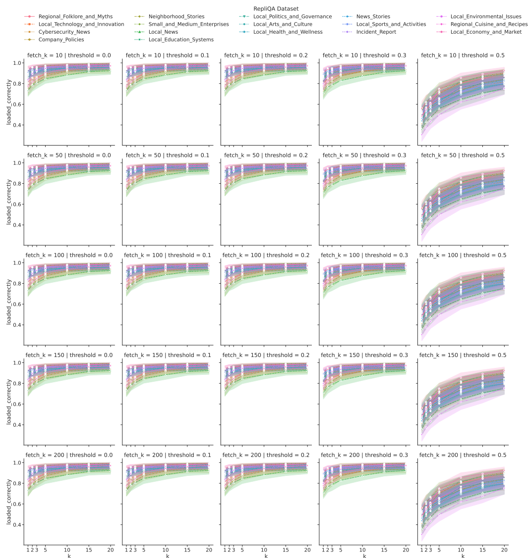
Figure C.4: RepliQA retrieval.
