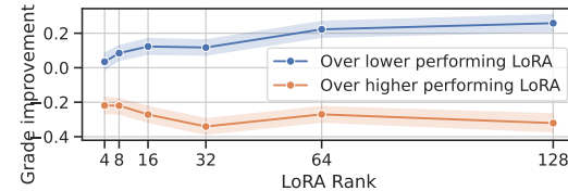
(b) Mixed LoRAs grade improvement on CS-COMBI.
