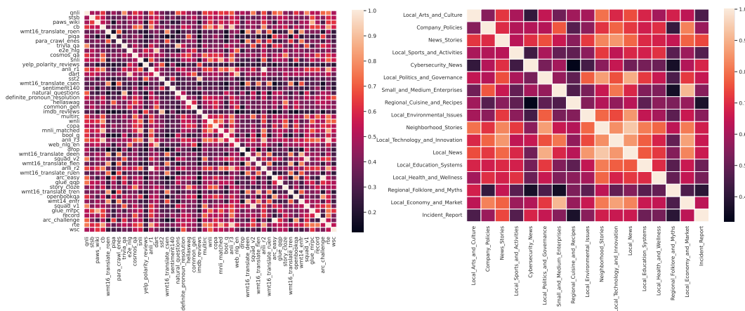
Figure B.4: All pair cosine similarities of Flan-v2 [21] and RepliQA [22] datasets.
