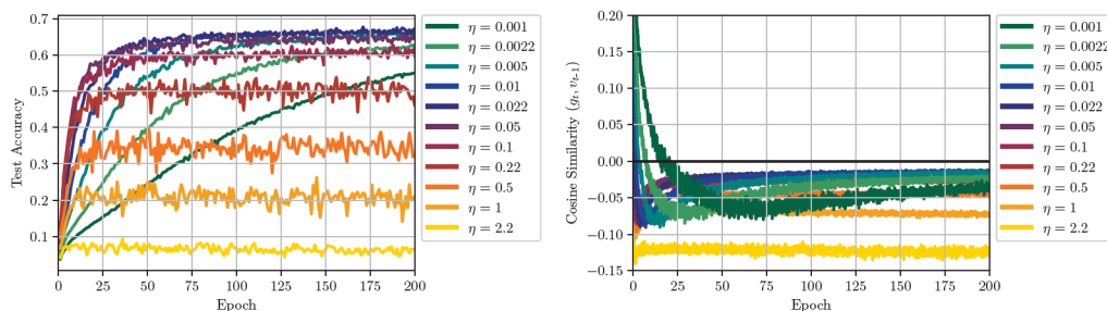
Figure A.5: WRN-16-4 on CIFAR100. Constant learning rate. Moving average over 50 iterations. Negative cosine similarity (and thus overshooting) even for very small learning rates. Runs with large learning rates still show overshooting when training is not possible anymore.
