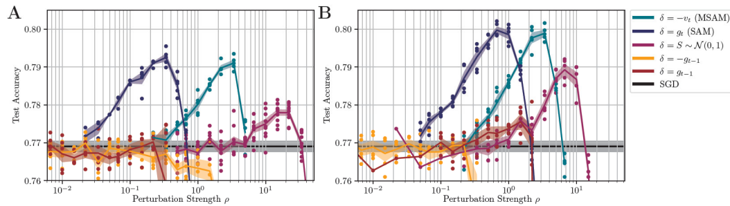
Figure A.9: Random perturbations and last gradient perturbations compared to SAM and MSAM. A: Absolute perturbations, B: Relative perturbations, i.e., scaled by |w_i| before normalization. All perturbations normalized by L2-norm and scaled by \rho . WideResNet 16-4 trained on CIFAR100. MSAM always better than other current gradient-independent perturbations.
