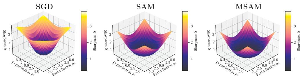
Figure A.13: 2D sharpness landscapes for two random filter-normalized perturbations (cf. Li et al. (2018)) as shown in Fig. 4C in 1D.
