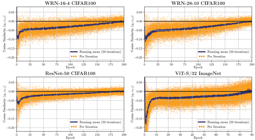
Figure A.3: Cosine similarity between momentum vector v_{t-1} and gradient g_t = \nabla L_{\mathcal{B}_t}(w_t) for different models/datasets. all with cosine scheduler
