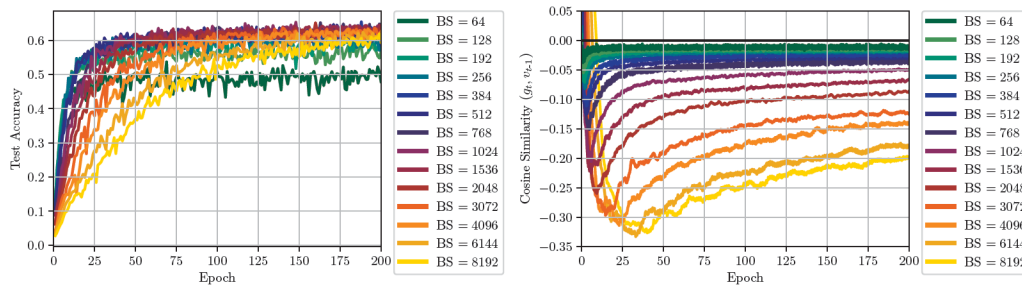
Figure A.7: WRN-16-4 on CIFAR100. Constant learning rate. Moving average over 50 iterations. While larger batch sizes result in less stochasticity, the cosine similarity is reduced. This supports that the negative slope is a property of the training-dataset loss landscape and not caused by limited sampling.
