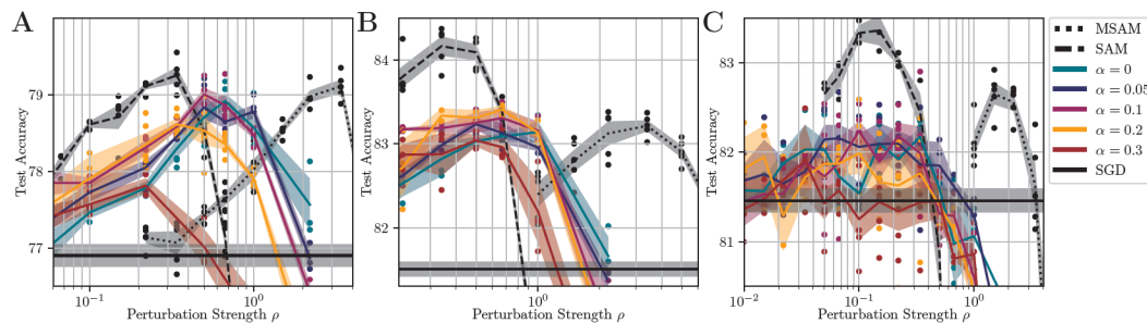
Figure A.14: Full results for \rho and \alpha search for lookSAM ( k = 5 ) on CIFAR100. Shaded cone: 68% CI. Dots: Random Seeds. A: WideResNet-16-4. B: WideResNet-28-10. C: ResNet-50.
