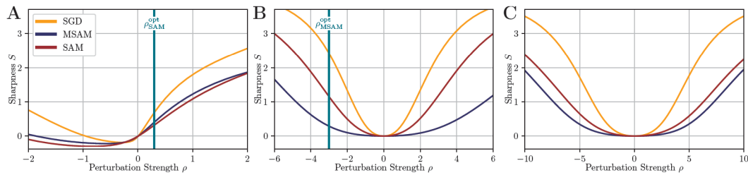
Figure 4: Sharpness (Eq. 3) after full training (200 epochs) for WideResNet-16-4 on CIFAR100 along different directions \epsilon scaled by \rho . A : Gradient direction (as used as perturbation in SAM). B : Momentum direction (as in MSAM). C : Random filter-normalized direction as in Li et al. (2018). Vertical line at \rho^{\text{opt}} marks values of optimal test performance (cf. Fig. A.15A). MSAM and SAM are reducing their respective optimization objective best while MSAM reaches the lowest sharpness along random directions.
