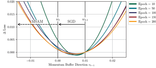
Figure A.2: Loss change (i.e. sharpness) in momentum buffer direction v_{t-1} during optimization. WRN-16-4 on CIFAR100 averaged over 30 runs. Minima are overshoot resulting in loss increase for further perturbations in negative momentum direction as done by MSAM. Effect even occurs for low (constant) learning rate of \eta = 0.01 used here while we use \eta = 0.5 in the main manuscript.
