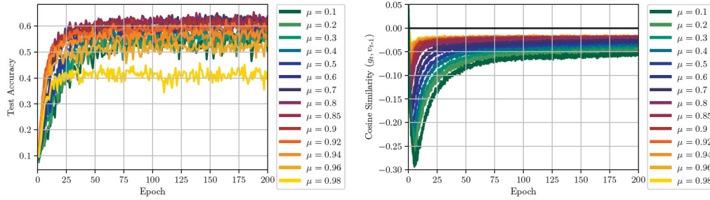
Figure A.6: WRN-16-4 on CIFAR100. Constant learning rate. Moving average over 50 iterations. Small \mu , i.e., faster forgetting of the momentum buffer, results in more overshooting.
