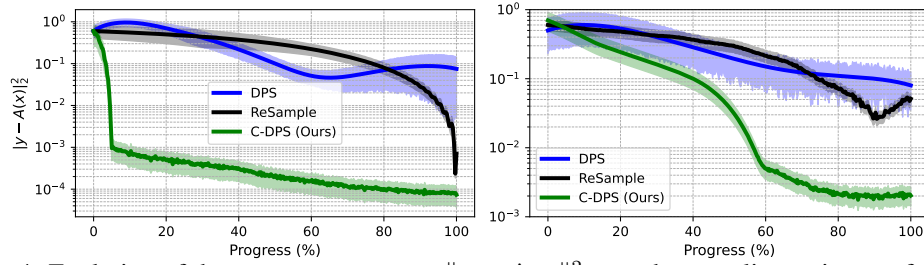
Figure 4: Evolution of the measurement error \|\mathbf{y} - \mathbf{A}\mathbf{x}_t\|_2^2 over the sampling trajectory for DPS, ReSample, and C-DPS on the FFHQ (left) and ImageNet (right) datasets.
