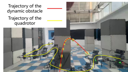
Figure 5: Real-world Experiment The quadrotor avoids the tennis ball thrown by experimenters during navigation.
