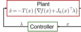
Figure 1: Control Perspective for Constrained Optimization
