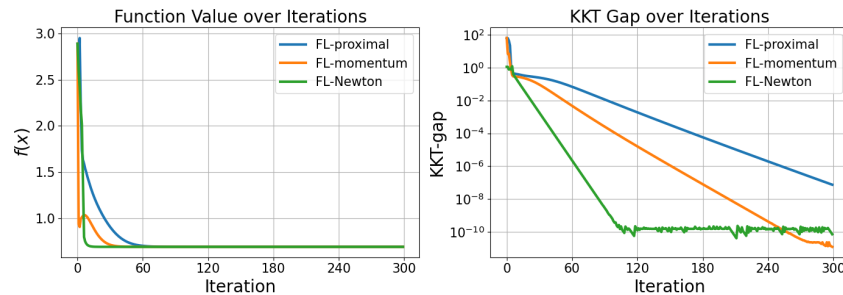
Figure 2: Result for Heterogeneous Logistic Regression
