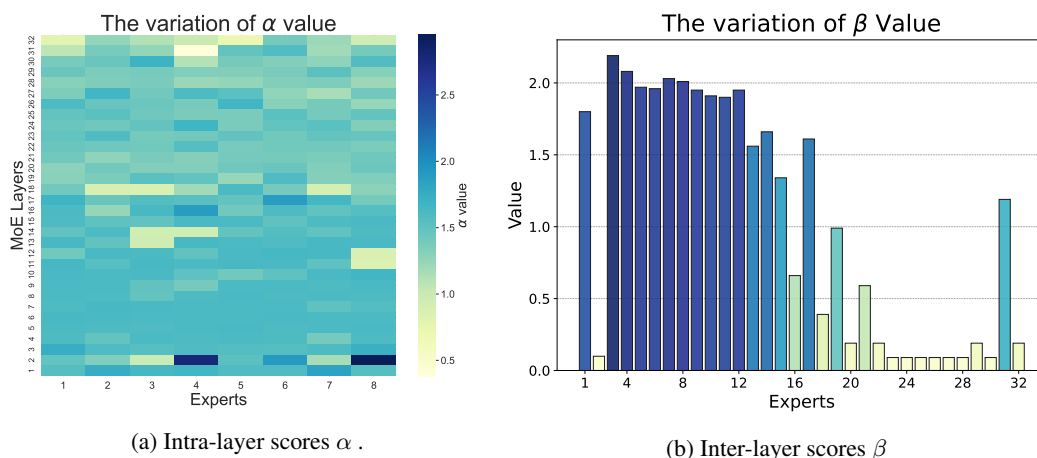
Figure 4: Visualization of values distribution for intra-layer scores \alpha and inter-layer scores \beta on Mixtral 8 \times 7B when r = 50\% .
