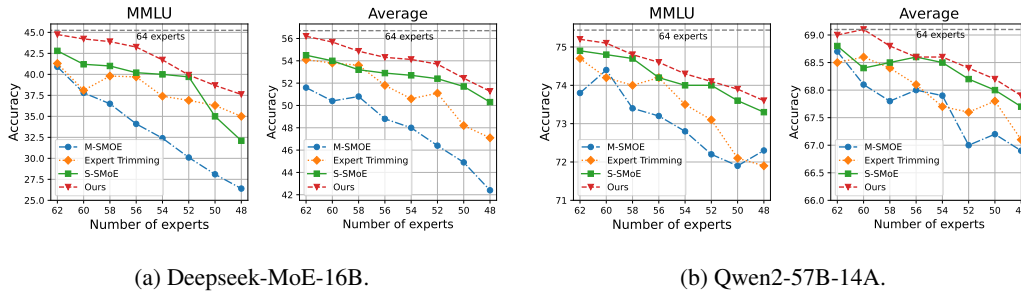
Figure 3: Zero-shot performance comparison on Deepseek-MoE-16B and Qwen2-57B-14A.
