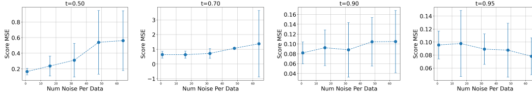
Figure 2: Score estimation error (mean \pm s.d.) versus the number of noise per data, i.e., k , for four noise levels, where lower error implies better score learning.
