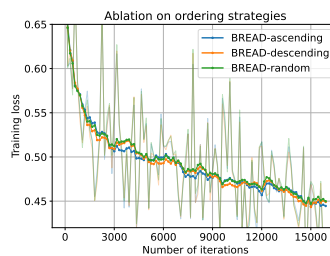
Figure 4: Ablation study on block ordering strategies
