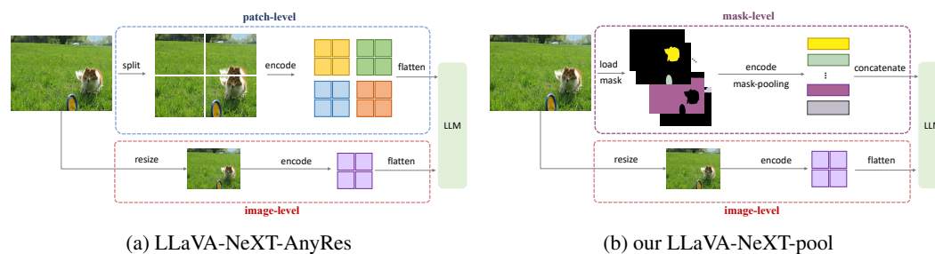
Figure 8: Comparison of LLaVA-NeXT and our proposed LLaVA-NeXT-pool.
