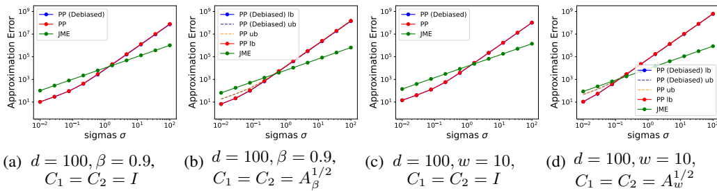
Figure 7: Expected error of second moment estimation with JME versus PP under different workload settings. The scenarios include exponential decay ( \beta = 0.9 ) and sliding window ( w = 10 ) workloads and d = 100, n = 1000 , both trivial and square root matrix factorization. In line with our analysis, incorporating matrix factorization significantly improves the quality of both methods, particularly in the high privacy regime.
