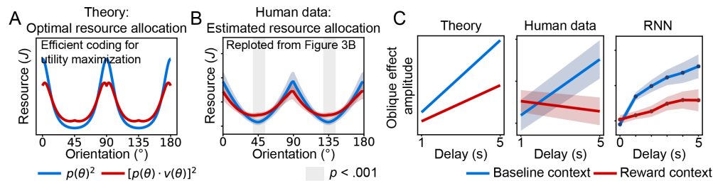
Figure 4: Utility maximization extension of efficient coding theory. (A) Optimal resource J for baseline context ( J_{\text{opt}} \propto p(\theta)^q ), and reward context ( J_{\text{opt}} \propto [p(\theta) v(\theta)]^q ). Here set q = 2 for illustration. (B) Resource allocation estimated from the behavioral data (5-sec delay) was consistent with the theoretical prediction (A). The shaded gray areas represent the clusters showing significant differences in resource between the two contexts (permutation test, p < .001 ). (C) Left: The optimal resource allocation predicts a stronger oblique effect in the baseline than in the reward context. In addition, the increment of the oblique effect over time is more rapid in the baseline context. These predictions are consistent with the behavioral data (middle) and the RNNs (right). Color shade error bar as the standard error.
