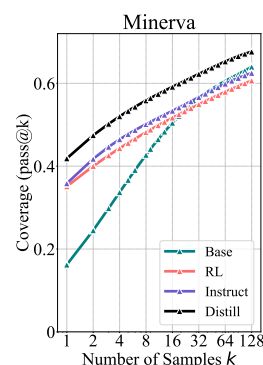
Figure 7: \text{pass}@k of base, Instruct, RLVR, and distilled models.
